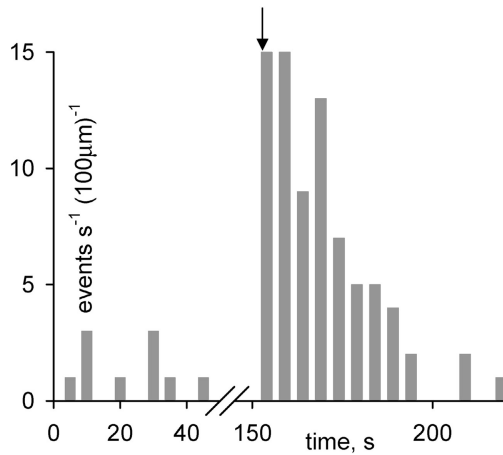
FIGURE 8. Evolution of event frequency after \text{Ca}^{2+} photorelease in the frog. Frequency (number of events per second and 100 \mu\text{m} ) in successive line scan images, 10 before and 15 after the flash, taken at 5-s intervals. The cell contained 1 mM NP-EGTA, at nominal [\text{Ca}^{2+}] of 100 \text{ nM} . The flash was applied at the beginning of a line scan, at arrow. Image identifier 082003a1.1-10, 082003a2.1-15
