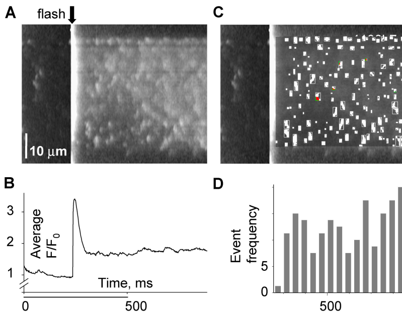
FIGURE 7. Fluorescence with synchronized flash photorelease of Ca 2+ . (A) Line scan of fluorescence in a frog fiber, synchronized with a 355-nm flash (at arrow). The cell was equilibrated with solution containing 1 mM NP-EGTA and 100 nM nominal [Ca 2+ ]. Fluorescence was normalized to its average before the flash. (B) Spatial average of fluorescence vs. time. Profiles like this, fitted in Fig. 1, are consistent with a peak of [Ca 2+ ] near 100 μM. The steady increase that follows the peak corresponds to ~80 nM above resting level. (C) Sparks located by the automatic detection program, which mark the image with boundaries of the suprathreshold "footprint" of each event. (D) Number of events detected in successive time bins of 40 ms, starting 40 ms after the flash. Image identifier 1030B7.1.
