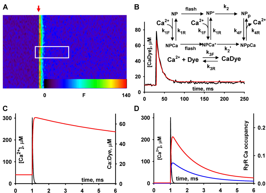
FIGURE 1. Calibrations of \text{Ca}^{2+} photolytic release. (A) Line scan of fluorescence of a saline containing caged \text{Ca}^{2+} (5 mM NP-EGTA and calcium added for a nominal [\text{Ca}^{2+}] of 150 nM) and fluo-3. xt image was acquired at 2 ms per line and 0.1428 \mu\text{m} per pixel. The white box covers 3.7 \mu\text{m} and 250 ms. At arrow, a 355-nm flash from a Nd:YAG laser was delivered via a tapered optic fiber of 200 \mu\text{m} end diameter. (B) Black trace: time course of spatial average of fluorescence within the box in A. Red: time course of [\text{CaDye}] (proportional to fluorescence) derived by numerical solution of a model of Ellis-Davies et al. (1996), represented in inset. (C) Time course of [\text{Ca}^{2+}] (black) and of [\text{CaDye}] (red), derived from the numerical solution, on expanded time scale. (D) Occupancy of a (activation) \text{Ca}^{2+} binding site, driven by the [\text{Ca}^{2+}] transient in black trace (reproduced from C). Blue and red traces are for [\text{Mg}^{2+}] of 1 and 0.4 mM, respectively. Parameters of photorelease model: k_{1F} = 0.017 \mu\text{M}^{-1} \text{ms}^{-1} , k_{1R} = 0.00136 \text{ms}^{-1} , k_2 =
