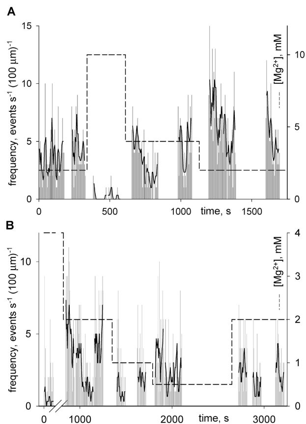
FIGURE 13. Dependence of spark frequency on cytosolic [Mg^{2+}] in the rat. Frequency in successive images vs. time. Dashed trace: nominal [Mg^{2+}] in perfusing solution. (A) Changes in a high [Mg^{2+}] range. (B) Changes in a low [Mg^{2+}] range. Note absence of systematic changes of frequency in B. Image identifiers: (A) 011301d; (B) 011701b.
