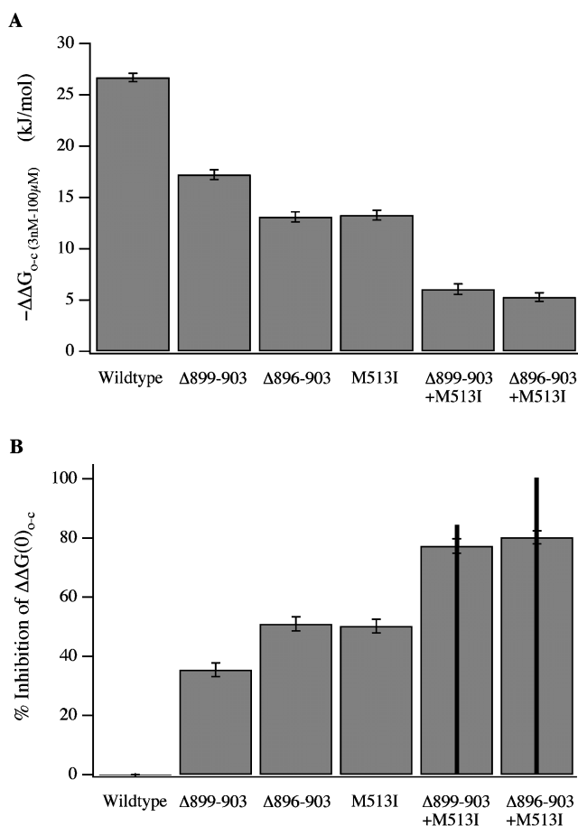
FIGURE 9. Additivity of mutations. (A) -\Delta\Delta G(0)_{oc} (3 nM to 100 \mu\text{M} [\text{Ca}^{2+}] ) is plotted for each channel type. (B) For each channel type is plotted (\Delta\Delta G(0)_{oc}(3\text{ nM to }100\text{ }\mu\text{M }[\text{Ca}^{2+}])_{\text{wild-type}} - \Delta\Delta G(0)_{oc}(3\text{ nM to }100\text{ }\mu\text{M }[\text{Ca}^{2+}])_{\text{mutant}}) / \Delta\Delta G(0)_{oc}(3\text{ nM to }100\text{ }\mu\text{M }[\text{Ca}^{2+}])_{\text{wild-type}} , which is the percent reduction in response to 100 \mu\text{M} [\text{Ca}^{2+}] caused by each mutation. Vertical black lines indicate the predictions of strict additivity, and are thus the sums of the bars for each individual mutant that contributes to a double mutant.
