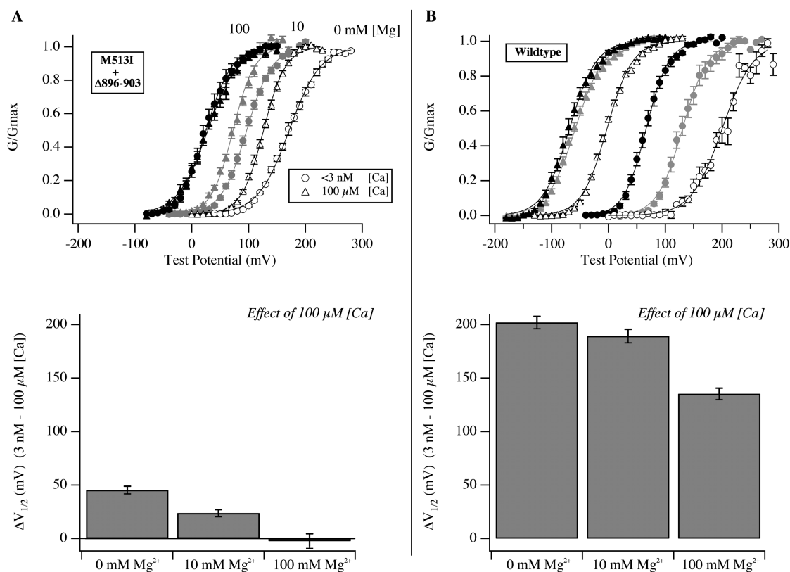
FIGURE 5. The remaining \text{Ca}^{2+} response of M513I+Δ896-903 is blocked by \text{Mg}^{2+} . (A) Top, G-V curves for the double mutant M513I+Δ896-903. Circles represent <3\text{ nM [Ca}^{2+}</math>. Triangles represent 100\text{ }\mu\text{M [Ca}^{2+}</math>. Open symbols indicate the absence of \text{Mg}^{2+}</math>. Grayed symbols indicate the presence of 10\text{ mM [Mg}^{2+}</math>. Darkened symbols indicate the presence of 100\text{ mM [Mg}^{2+}</math>. Each curve has been fitted with a Boltzmann function. Bottom, plots of the change in V_{1/2} as [\text{Ca}^{2+}]</math> is increased from <3\text{ nM}</math> to 100\text{ }\mu\text{M}</math> in the presence of either 0, 10, or 100 mM [\text{Mg}^{2+}</math>. (B) Same experiment as in A except the wild-type channel was used. Mean V_{1/2} values were determined from Boltzmann fits to the data from each experiment individually.
