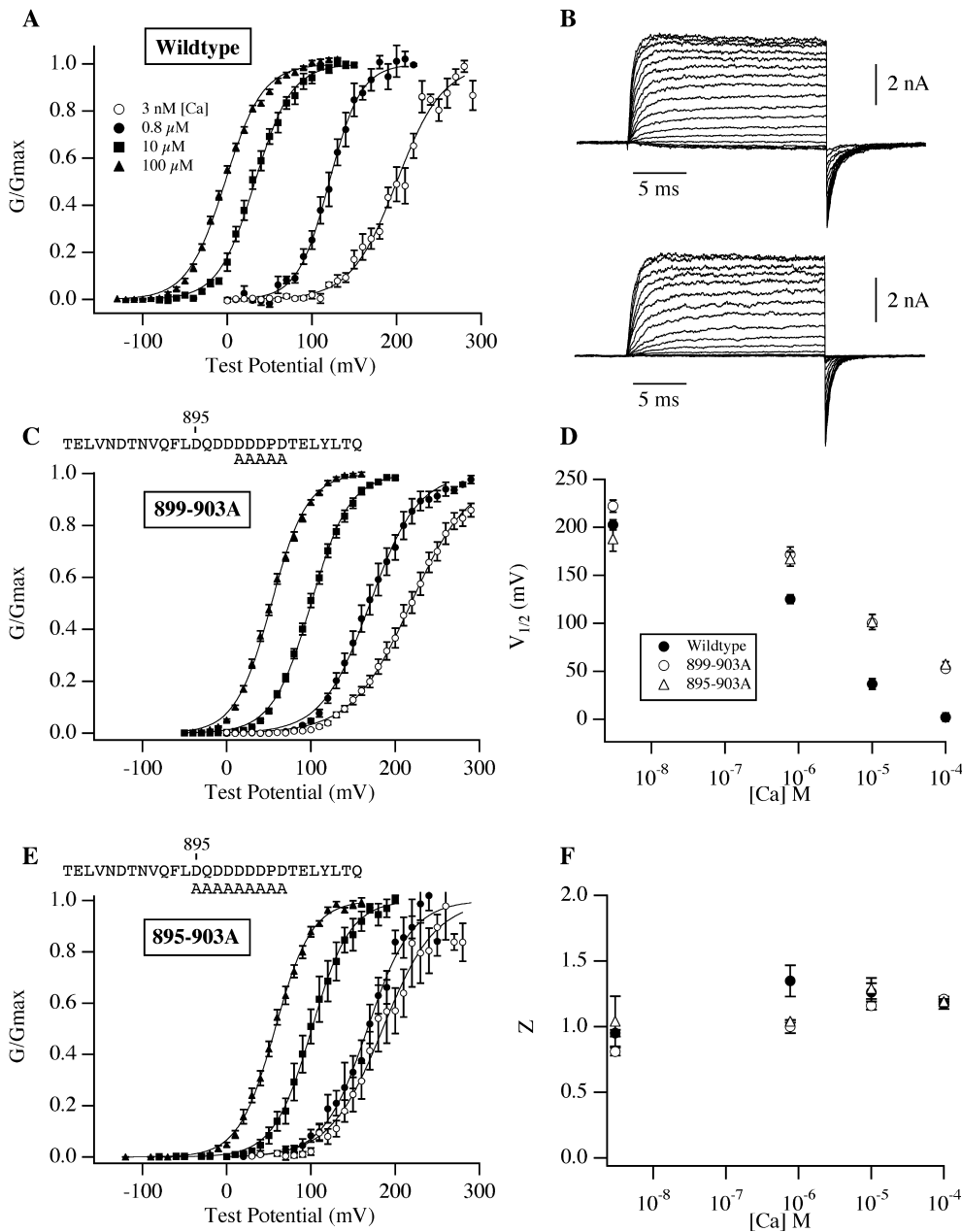
FIGURE 2. \text{Ca}^{2+} bowl mutations reduce mSlo's \text{Ca}^{2+} response. (A) G-V relations determined from inside-out Xenopus oocyte macropatches expressing the mSlo protein. [\text{Ca}^{2+}]_i are as indicated on the figure. (B) Wild-type (top) and mutant (895–903A; bottom) mSlo current families recorded with voltage steps to between -40 and 130 mV with 100 \mu\text{M} internal [\text{Ca}^{2+}]_i . Tail potentials are -80 mV; holding potentials are -120 mV (top) and -100 mV (bottom). (C) G-V relations determined from patches expressing the \text{Ca}^{2+} bowl mutant 899–903A. The residues mutated to alanine are indicated above the plot. (D) Half maximal activation voltage ( V_{1/2} ) vs. [\text{Ca}^{2+}]_i plots for the data in panels A, C, and E. The points plotted are average parameter values determined from experiments fitted individually with a Boltzmann function (see Table I for values). Symbols represent channel type as indicated on the figure. (E) G-V relations determined from patches expressing the \text{Ca}^{2+} bowl mutant 895–903A. (F) Apparent gating valence ( z ), determined from Boltzmann fits, plotted as a function of [\text{Ca}^{2+}]_i (see Table I for values). Symbols represent channel type as in D. Error bars in this and subsequent figures represent standard error of the mean.
