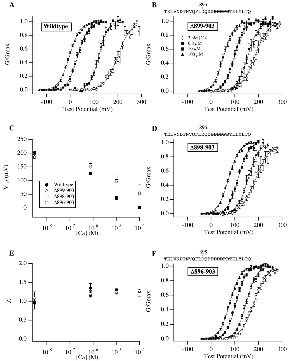
FIGURE 3. Many Ca 2+ bowl mutants behave similarly. (A) Wild-type G-V relations determined at a series of [Ca 2+ ] as in Fig. 2. (B) G-V relations for the mutant Δ899–903. The residues deleted are indicated above the plot with a line drawn through them. (C) V 1/2 vs. [Ca 2+ ] plots for the channels in A, B, D, and F (see Table I for values). (D) G-V relations for the mutant Δ898–903. (E) z vs. [Ca 2+ ] plots for the channels in A, B, D, and F (see Table I for values). Symbols represent mutants as indicated in C. (F) G-V relations for the mutant Δ896–903. In A, B, D, and F symbols represent [Ca 2+ ] as indicated in B.
