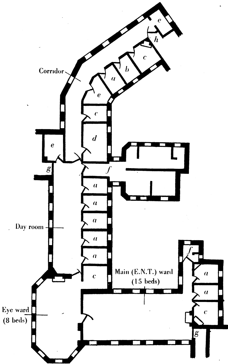
Fig. 1. Plan of combined E.N.T. Eye ward.
