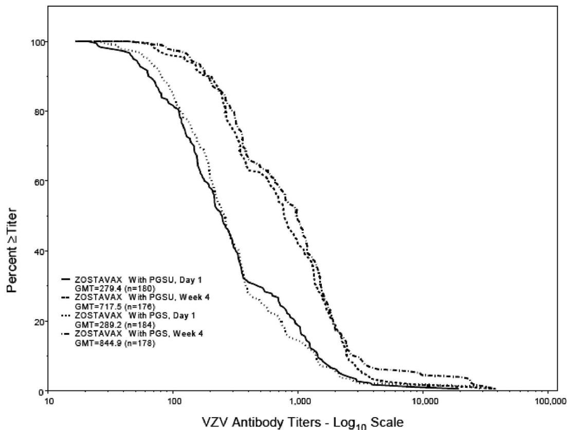
FIG. 2. Reverse cumulative distribution of VZV-specific antibody titers at prevaccination and 4 weeks postvaccination by vaccination group.
