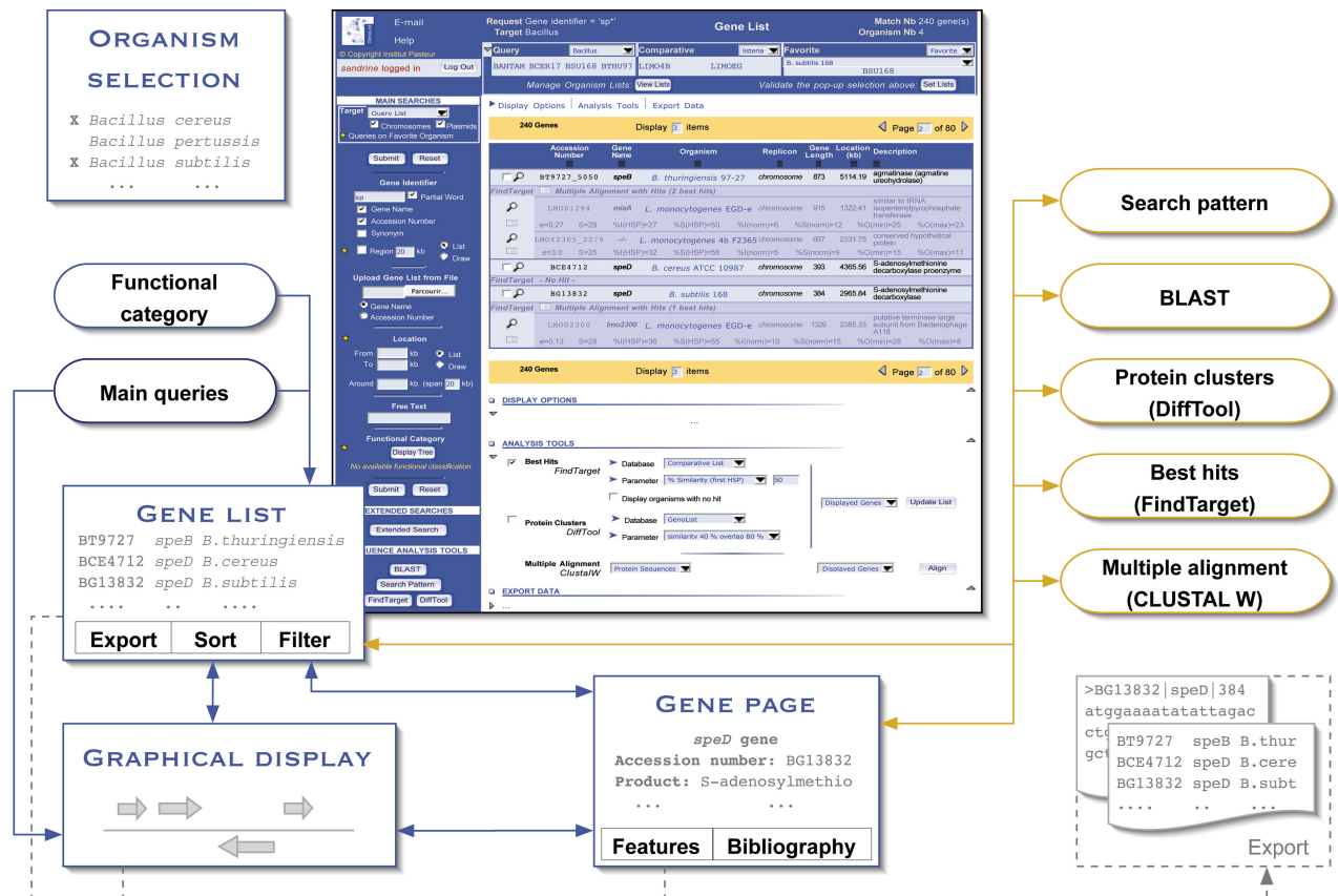
Figure 1. Data and functionality integration in the GenoList environment. The first step consists in selecting species of interest ('Organism selection' panel). The central component of the application is the 'Gene list' panel (shown in the screen capture). Search outputs are presented there ('Main queries' and 'Functional category'—blue rounded boxes), and results of sequence analysis tools ('Search pattern', 'BLAST', 'DiffTool' and 'FindTarget'—yellow rounded boxes), which are displayed using specific layouts (e.g. BLAST reports), can also be converted to standard 'Gene lists'. This panel acts as a hub since it gives access to many additional features ('Gene page', 'Graphical display' and 'Export'), and it allows the user to bounce back to the sequence analysis tools from either one single gene or a subsection of the gene list. The screen capture illustrates the visualization of best hits of selected genes in a standard 'Gene list'.
