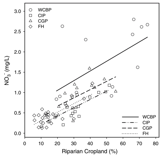
Fig. 7 Example of typically observed relationships between riparian land cover and water chemistry parameters among the four ecoregions analyzed (WCBP, Western Corn Belt Plains; CGP, Central Great Plains; FH, Flint Hills; CIP, Central Irregular Plains). The percentage of riparian cropland in the watersheds is plotted versus in-stream NO 3 - concentrations. Slopes of regression lines fitted through each of the four ecoregions were not significantly different
