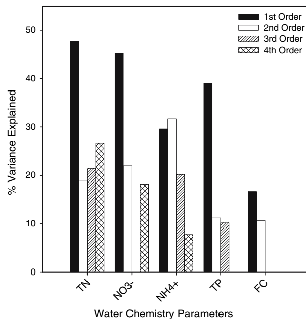
Fig. 5 Variance in water chemistry variables ( R^2 values) explained by riparian land cover adjacent to different sized streams within watersheds. Analyses performed with a subset of 39 fourth-order watersheds; TN analyses performed with 38 fourth-order watersheds. Comparisons between riparian land cover and AT and maximum DO concentrations were not significant and are not presented
