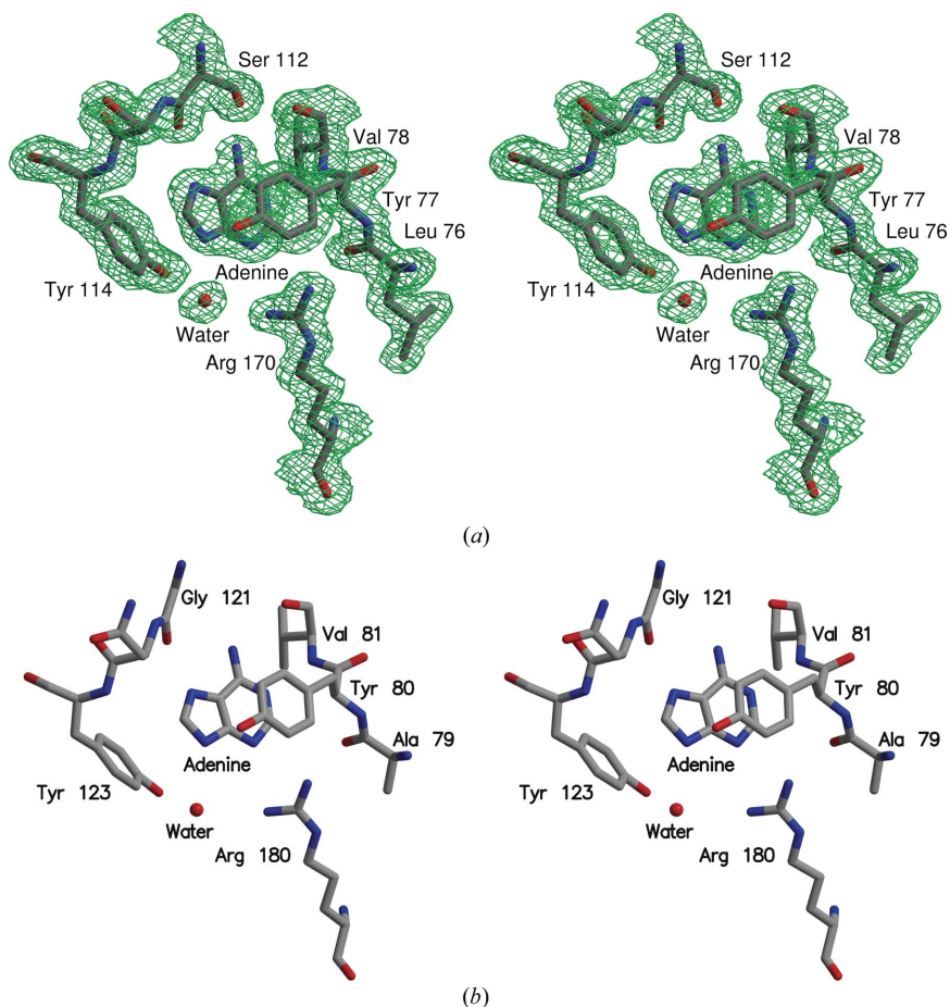
Figure 1 (a) Stereoview of the electron density for adenine bound at the active site of Stx2. The 2|F_o| - |F_c|, \alpha_c map was calculated using the data from Stx2 crystallized with adenosine and is contoured at 1\sigma . The model is shaded according to atom type: grey for carbon, blue for nitrogen and red for oxygen. This figure was drawn using Xfit (McRee, 1999) and RASTER3D (Merritt & Bacon, 1997). (b) Stereoview of adenine bound at the active site of the A chain of ricin. For ease of comparison, the orientation is similar to that used in (a).
