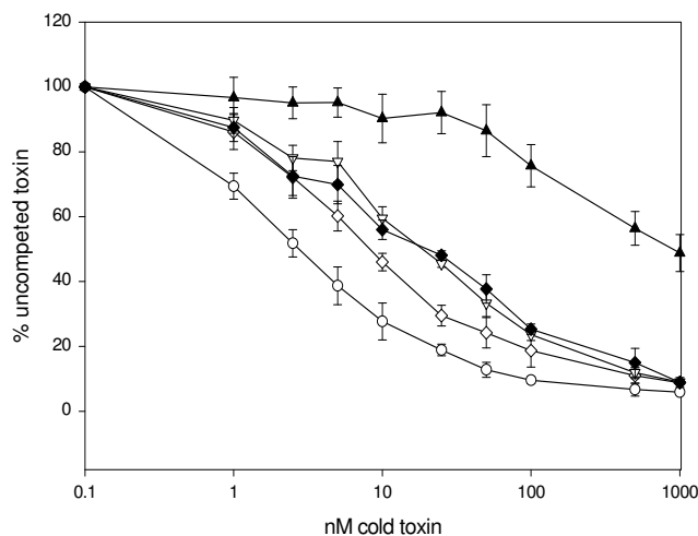
Figure 2 Competition with labeled CryIAa and mutant toxins to B. mori brush border membrane vesicles (BBMV) (bars represent error of n = 4). Cry1Aa wild type protein, (-); F313A mutant protein, (◇-◇); F333A-F335A, mutant protein (▽-▽); F461A mutant protein, (◆-◆); and, F328A mutant protein, (-). % uncompetited toxin indicates the % of labeled toxin remaining bound to BBMV in the presence of unlabeled cold toxin competitor.
