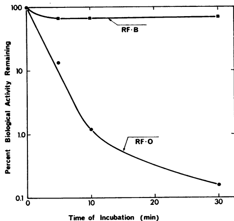
FIG. 1.—Effect of B/41 dialyzed ammonium sulfate fraction upon fd RF·O and fd RF·B. Reaction mixtures without protein were prepared as described in Materials and Methods , prewarmed, mixed with the dialyzed ammonium sulfate fraction from strain B/41, and incubated at 37° for the times indicated. After incubation they were chilled in ice and 15 \mu liters of 0.2 M EDTA was added. The zero time samples were mixed with EDTA before the addition of protein and showed no loss of activity compared to untreated RF.
