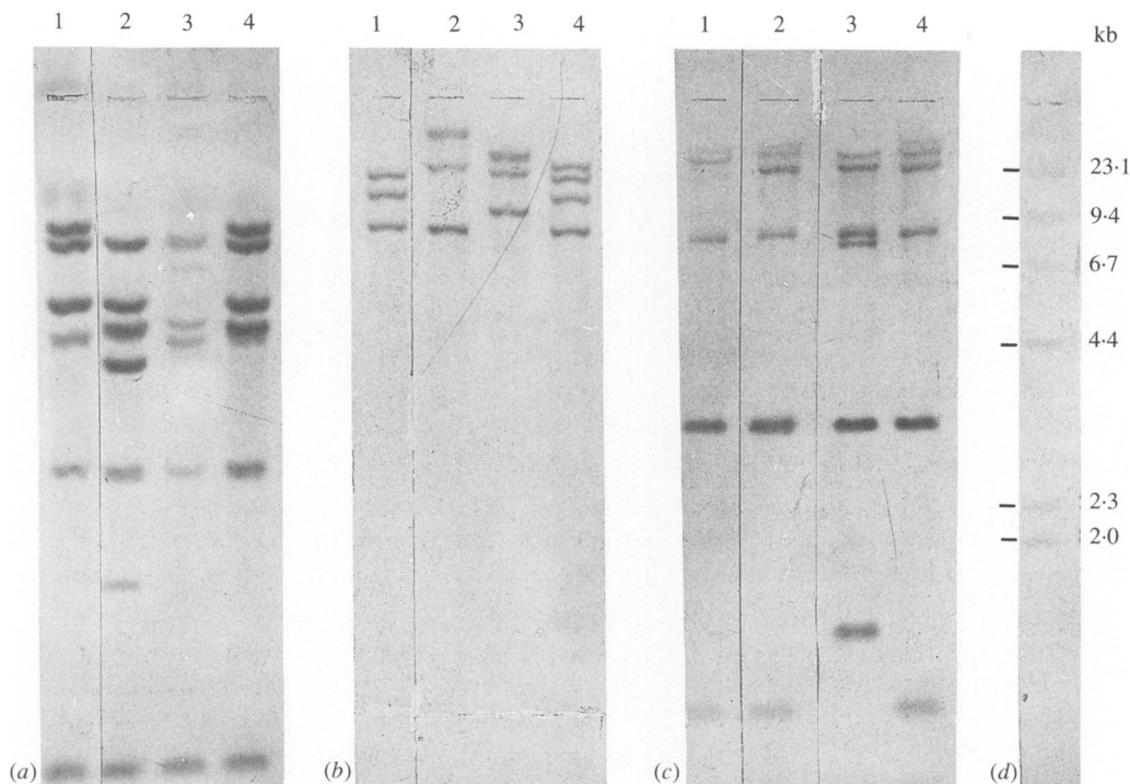
Fig. 4. Southern blot patterns of restriction digests of DNA from P. aeruginosa O 12 strains hybridized with a biotinylated cDNA probe transcribed from total rRNA from P. aeruginosa serotype strain O 12: (a) Sma I, (b) Eco RI, (c) Hind III (d) Hind III digest of biotinylated lambda phage DNA. Lane 1, strain no. 12. 2, Strain no. 20. 3, Serotype strain. 4, Strain nos. 1, 2, 4, 6, 8, 10, 14, 16, 17, 19, 25 (see Table 3 for origin).
