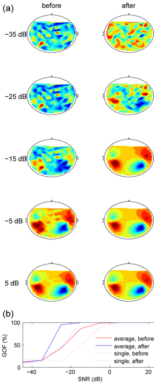
Fig. 4. (a): Topographies of synthetic “auditory M100” activity produced by a two-dipole model at various values of SNR, before and after denoising. (b) Goodness-of-fit (GOF) as a function of SNR. Full lines: GOF of average over 10 repeats. Dotted lines: average of GOFs of a single repeat.
