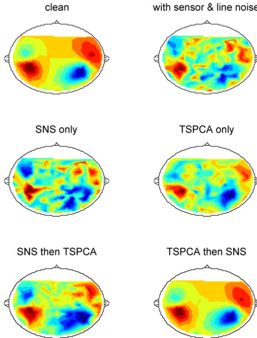
Fig. 5. Combining SNS and TSPCA (de Cheveigné and Simon 2007). Top left: field distribution at the peak of a simulated M100 response based on a two-dipole model. Top right: same superimposed on a mixture of simulated environmental noise and sensor noise (in equal proportions) at SNR=-18 dB. Middle: result of applying SNS alone (left) or TSPCA alone (right). Bottom: result of applying SNS followed by TSPCA (left) or TSPCA followed by SNS (right).
