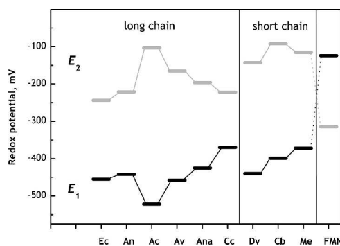
Figure 1. The E_1 , sq/hq, and E_2 , q/sq, midpoint potentials for long- and short-chain flavodoxins from different sources at pH 7.0, in mV. From left to right: E. coli (Hoover and Ludwig 1997), A. nidulans (Hoover et al. 1999), A. chroococcum (Deistung and Thorneley 1986), A. vinelandii (Steensma et al. 1996), Anabaena 7120 (Paulsen et al. 1990), C. crispus (Sykes and Rogers 1984), D. vulgaris (Curley et al. 1991), C. beijerinckii (Mayhew 1971), M. elsdenii (Mayhew et al. 1969), and finally, FMN free in solution (Anderson 1983), with E_1 and E_2 inverted with respect to the flavodoxins. For the cases where the potentials were not measured at pH 7.0, a change of -59 mV/pH unit was applied to estimate E_2 ( E_1 was assumed to be pH independent above pH 7.0).
