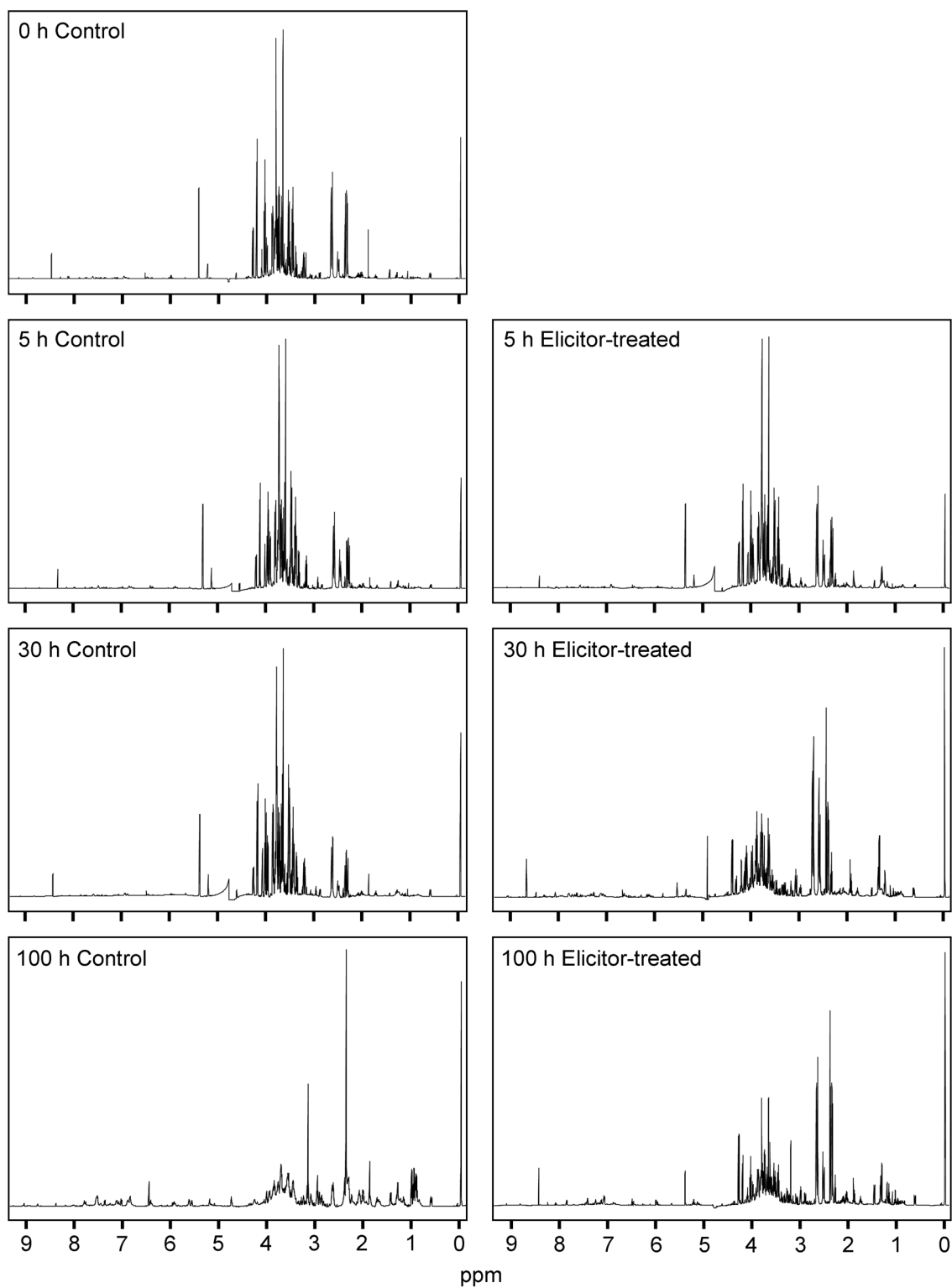
Figure 1 ^1\text{H} NMR spectra of \text{D}_2\text{O} extracts from control and elicitor-treated opium poppy cell culture collected 0, 5, 30 and 100 h post-elicitation. 2,2-Dimethyl-2-silapentane-5-sulfonate (DSS) was used as an internal standard. The peak height of DSS, which was set at 0 ppm, is equivalent for all spectra.
