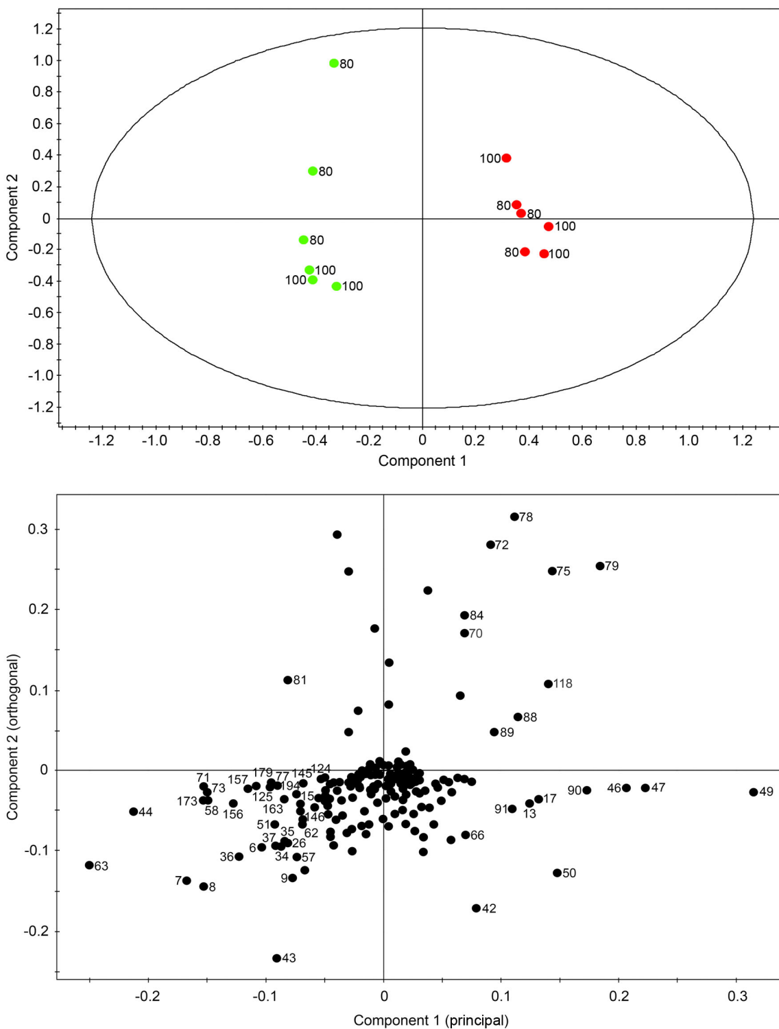
Figure 5 Scores (A) and corresponding loadings plot (B) of orthogonal partial least-squares-discriminant analysis (OPLS-DA) on 1 H NMR spectra for D 2 O extracts of control (green) and elicitor-treated (red) opium poppy cell cultures collected at 80 and 100 h post-elicitation. The ellipse in A represents the Hotelling with 95% confidence. Numbers beside data point on the loadings plot correspond to specific bins used in the analysis.
