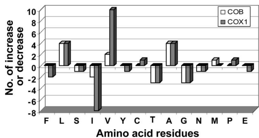
FIG. 3. Editing-mediated increase (+) or decrease (-) in the content of the 20 amino acid substituents of COB and COX1. Amino acids are denoted by their standard one-letter abbreviations.
