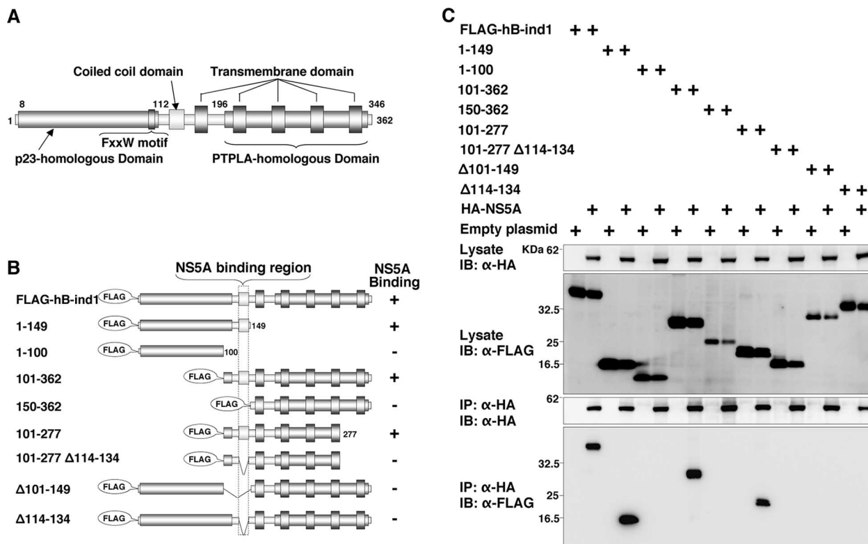
FIG. 2. Determination of the NS5A-binding region in hB-ind1. (A) Structure and functional domains of hB-ind1. (B) Deletion mutants of hB-ind1 used in this study and the results of binding to NS5A. N-terminally FLAG-tagged hB-ind1 mutants encoding the region from residue 1 to 149, 1 to 100, 101 to 362, 150 to 362, or 101 to 277 were designated 1-149, 1-100, 101-362, 150-362, or 101-277, respectively. An N-terminally FLAG-tagged hB-ind1 mutant spanning the region from residue 101 to residue 277 but lacking residues 114 to 134 was designated 101-277 Δ114-134. In addition, N-terminally FLAG-tagged hB-ind1 mutants lacking the region from 101 to 149 or from 114 to 134 were designated Δ101-149 or Δ114-134, respectively. The coiled-coil domain was located at residues 114 to 134. Each mutant gene was inserted into pEF FLAGGs pGKpuro. A summary of immunoprecipitation results is given on the right. (C) Each hB-ind1 mutant was coexpressed with Con1 HA-NS5A in 293T cells, immunoprecipitated with an anti-HA antibody, and analyzed by Western blotting with an anti-FLAG antibody. As a negative control, an empty plasmid was used instead of the plasmid encoding HA-NS5A. The anti-HA antibody did not recognize FLAG-tagged hB-ind1 or its mutants.
