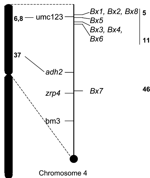
Figure 7. The genes Bx1 to Bx8 are located on the short arm of chromosome 4. Bx7 is about 35 cM distal to Bx6 . Bx1 to Bx6 and Bx8 map within 6 cM. The OMT Zrp4 maps at position 49; the maize gene Bm3 is located in position 61.7. The positions are given with respect to the Genetic 2005 map for chromosome 4 by E. Coe (www.maizegdb.org). Bold numbers refer to centiMorgan.
