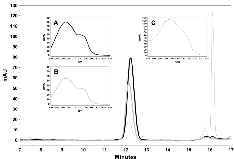
Figure 3. Benzoxazinoids in Bx6 mutant plants. Benzoxazinoids were isolated from mutant and wild-type plants (thick black line, mutant with insertion at position 1; thick gray line, mutant with insertion at position 4; thin black line, wild type; Frey et al., 2003) and analyzed as described in "Materials and Methods." DIBOA-glc is the predominant benzoxazinoid in the mutant. The spectra of the respective main peaks are displayed in the inserts. A and B, DIBOA-glc. C, DIMBOA-glc. mAU, Milli absorption units.
