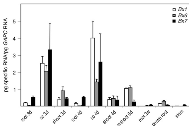
Figure 6. Expression of DIMBOA-glc biosynthesis genes. Three- and 4-d-old etiolated seedlings of line B73 were dissected in root, scutellar node and mesocotyl (sc), and shoot (leaves and coleoptile); after 6 d, mesocotyl, leaves, and coleoptile were pooled (mshoot). Tissues of older plants were taken after 3 weeks (root) and 10 weeks. Steady-state mRNA levels were measured by real-time reverse transcription-PCR using gene-specific primer pairs. GAPC mRNA quantities were determined in parallel and used for normalization.
