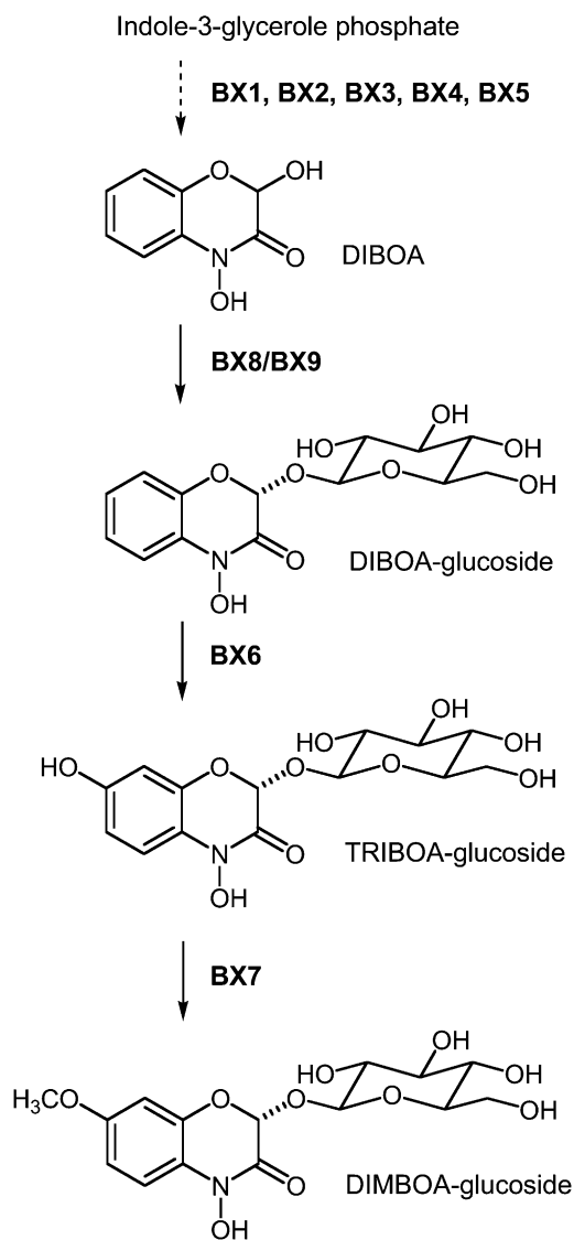
Figure 1. Enzymes and intermediates of DIMBOA-glc biosynthesis in maize. Conversion of indole-3-glycerole phosphate to indole by the enzyme BX1 represents the branch point from primary metabolism. The introduction of four oxygen atoms into the indole moiety that yields DIBOA is catalyzed by four cytochrome P450-dependent monooxygenases, BX2 to BX5. The resulting DIBOA is glucosylated by the UDP-glucosyltransferases BX8 and BX9. Hydroxylation in position C-7 of the glc is catalyzed by the 2ODD BX6. The final step of the pathway is the O -methylation of TRIBOA-glc by BX7 to produce DIMBOA-glc.
