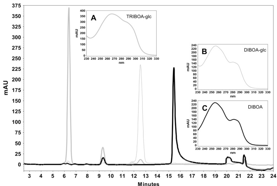
Figure 2. Analysis of BX6 enzyme activity using heterologously expressed protein and the substrates DIBOA and DIBOA-glc. Overlay of the HPLC traces. The inserts A, B, and C depict the spectra of the respective main peaks. Thick gray line: enzyme assay using DIBOA-glc as a substrate; the substrate is almost completely converted to TRIBOA-glc (spectrum A). Thick black line: enzyme assay with DIBOA as a substrate (spectrum C); no conversion is detected. Thin black line: incubation of DIBOA-glc under assay conditions without enzyme (spectrum B). Assay conditions were described in "Materials and Methods"; incubation time was 30 min. mAU, Milli absorption units.
