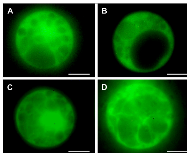
Figure 4. Subcellular localization of BX6. The fusion protein BX6part-GFP-BX6 is located in the cytoplasm of the cell. No GFP signal is detected in the vacuole. A and C, Control 2 \times 35S promoter-GFP. B and D, BX6part-GFP-BX6 fusion. A and B, Transient expression. C and D, Transgenic plants. The bar equals 10 \mu\text{m} .
