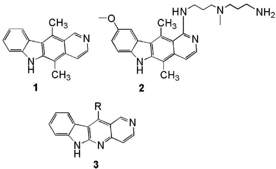
Figure 1. Ellipticines.
