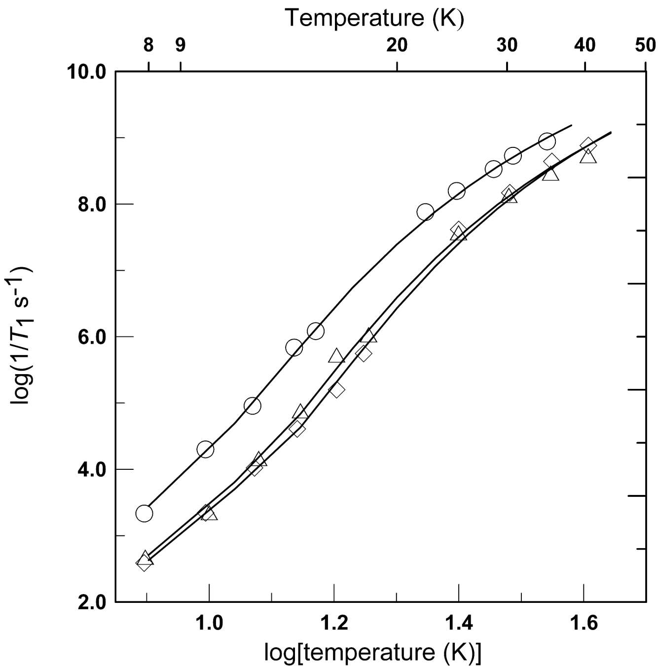
Figure 5. Temperature dependence of spin-lattice relaxation rates for two-electron reduced [4\text{Fe-4S}]^+ in Rhodobacter (○), porcine (◇) and human (△) ETF-QO. Values were measured by inversion recovery (8 to 16 K) or calculated from the temperature contribution to the lineshape (22 to ~40 K). The values of T_1 are averages along the g_x , g_y , and g_z turning points. The solid lines through the data are the fit functions calculated using the model in (Eq. (2)) and the parameters in Table 2. Samples are in 0.1 M Tris HCl, pH 7.8, containing 8 mM CHAPS and 40% glycerol.
