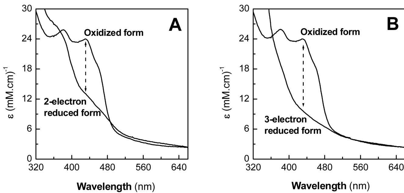
Figure 1. The absorption spectra of the oxidized, and 2- and 3-electron reduced species of Rhodobacter ETF-QO. The dashed double-headed arrow indicates the wavelength for which the change in molar absorptivity is reported. Samples are in 20 mM Hepes( \text{K}^+ ), pH 7.8, containing 30% glycerol. \Delta\epsilon_{430\text{ nm}} = 4.9\text{ mM}^{-1}\text{cm}^{-1}/\text{electron equivalent} .
