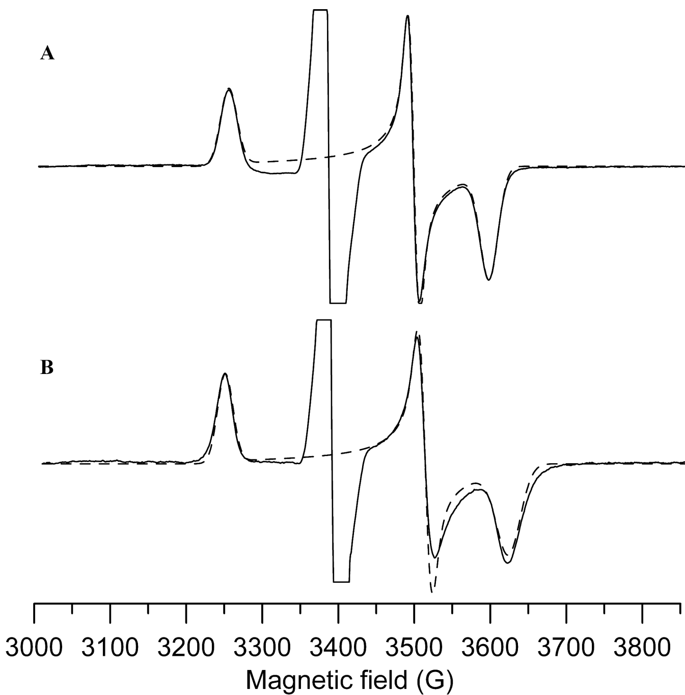
Figure 4. 9.49 GHz CW spectra of two-electron reduced porcine (A) and Rhodobacter (B) ETF-QO recorded at 15 K. The samples are in 0.1 M Tris HCl, pH 7.8, containing 8 mM CHAPS and 40% glycerol. Dashed lines are simulations calculated using the program MONMER.
