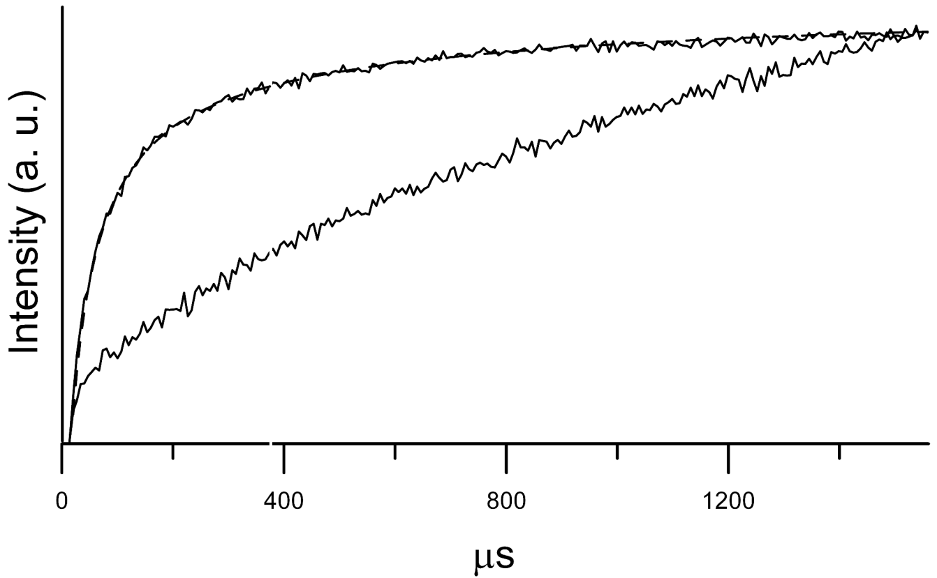
Figure 3. Inversion recovery curves for 2-electron reduced porcine ETF-QO ( upper curve ) and ETF ( lower curve ) at 36 K. The dashed line is a simulated curve calculated with MENOSR for an interspin distance of 19 Å. Samples are in 0.1 M Tris HCl, pH 7.8, containing 8 mM CHAPS and 40% glycerol.
