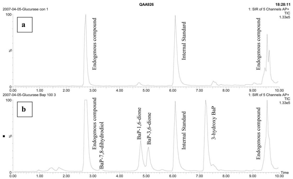
Fig. 3. Chromatogram of: (a) a control F. heteroclitus bile sample after glucurase digestion; (b) a BaP (100 \mu\text{g/L} ) exposed F. heteroclitus bile sample after glucurase digestion.
