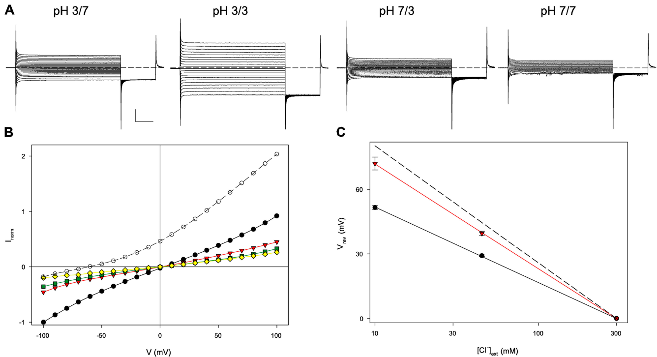
Figure 2. Loss of H^+ coupling in E203Q. (A) Currents mediated by E203Q in symmetrical 300 mM Cl^- , with or without a 4-unit pH gradient. A 3-s voltage pulse ( -100 to +100 mV in 10-mV steps) was applied from a holding potential of 0 mV, followed by a 1-s tail pulse to -100 mV. Dashed line marks zero current. (B) I-V curves, normalized to the current in the same bilayer at -100 mV in symmetrical pH 3.0 and 300 mM Cl^- . Open circles, wild type, pH 3.0/pH 7; black circles, E203 pH 3/pH 3; red triangles, E203 pH 3.0/pH 7; green squares, E203 pH 7/pH 3; yellow triangles, E203 pH 7.0/pH 7. Gradients are indicated by convention cis/trans sides of planar bilayer, with the trans side defined as zero voltage. (C) Reversal potential, V_{rev} , as a function of [Cl^-] for wild type (black circles) and E203Q (red triangles); dashed line is Nernst potential predicted for ideal Cl^- selectivity.
