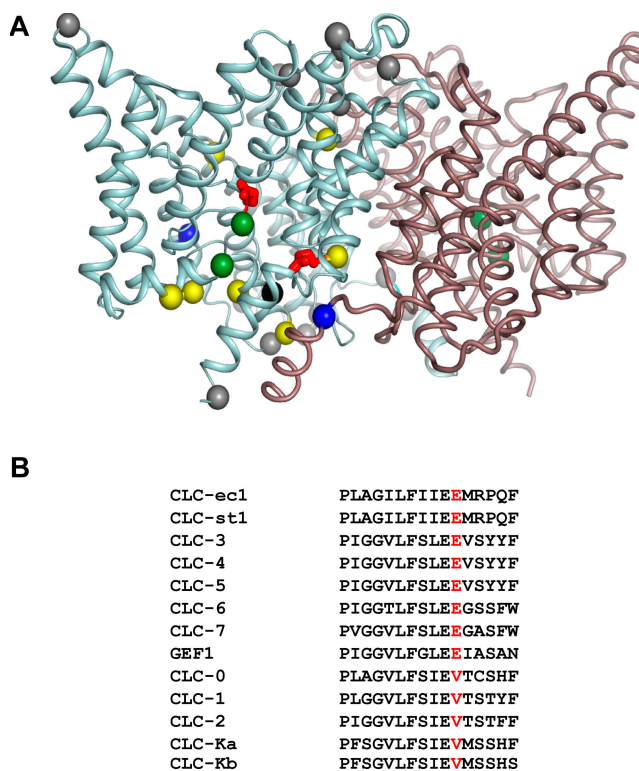
Figure 1. Carboxylates in CLC-ec1. (A) Ribbon representation of the CLC-ec1 dimer, view from within the membrane, with extracellular side up. \alpha carbons of the carboxylate residues mutated here are shown for a single subunit as yellow spheres, except for E148 and E203 (red), and E113 (black); gray spheres mark carboxyl residues that are not studied here, and green spheres designate \text{Cl}^- ions. Also shown are R28 and K131 (blue). (B) Sequence alignment of the PIGG-pen region, with E203 equivalent indicated in red. Genes listed are of human origin except for CLC-0 ( Torpedo marmorata ), CLC-ec1 ( E. coli ), CLC-st1 ( Salmonella typhimurium ), and GEF1 ( Saccharomyces cerevisiae ).
