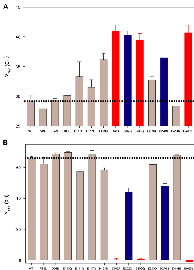
Figure 4. H^+/Cl^- coupling for CLC-ec1 mutants. Reversal potentials of indicated mutants in presence of (A) a Cl^- gradient (300 mM/45 mM) at symmetrical pH 3.0 or (B) a pH gradient (3/7) at symmetrical 300 mM Cl^- . Dotted lines represent wild-type values under the same conditions. Data for wild type and E148A taken from Accardi et al. (2004); EA/EQ denotes the double mutant E148A/E203Q. Colored bars indicate mutants with H^+ transport inhibited completely (red) or partially (blue).
