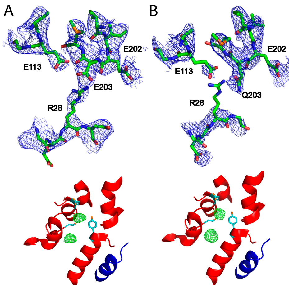
Figure 5. Crystal structure and halide binding. (A) Wild type; (B) E203Q. Top panel, 2F_o - F_c electron density maps (blue) contoured at 1.2 \sigma , with protein model shown in stick representation. Wild-type map was calculated to 3.3 \text{ \AA} resolution from deposited structure factors (accession no. 1OTS). Bottom panel, anomalous difference density maps (green) of crystals grown in NaBr, determined from data collected at the \text{Br}^- absorption edge, contoured at 5 \sigma , with the same wild-type protein model (1OTS) shown for both maps, with subunit A in red and subunit B in blue.
