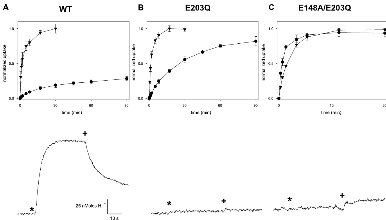
Figure 3. Fluxes of \text{Cl}^- and \text{H}^+ . Liposomes reconstituted with CLC-ec1 (1–5 \mu\text{g}/\text{mg} lipid) were assayed for either ^{36}\text{Cl}^- uptake or \text{Cl}^- -driven \text{H}^+ pumping. Top panels, ^{36}\text{Cl}^- uptake at pH 7.0 (circles) and pH 4.5 (triangles) for WT (A), E203Q (B), and E148A/E203Q (C). Lower traces show \text{H}^+ flux assays, upward deflection indicating increase in pH of the liposome suspension. Additions of 1 \mu\text{M} valinomycin or FCCP are denoted by * and +, respectively.
