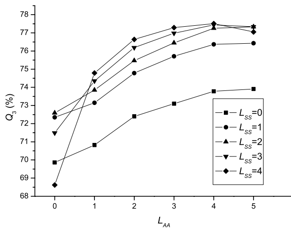
Figure 1 The influence of window sizes on the Q_3 of DBN. L_{AA} and L_{SS} are window sizes for profile and secondary structure, respectively. The results are obtained by testing DBN sigmoid on the SD576 dataset.
