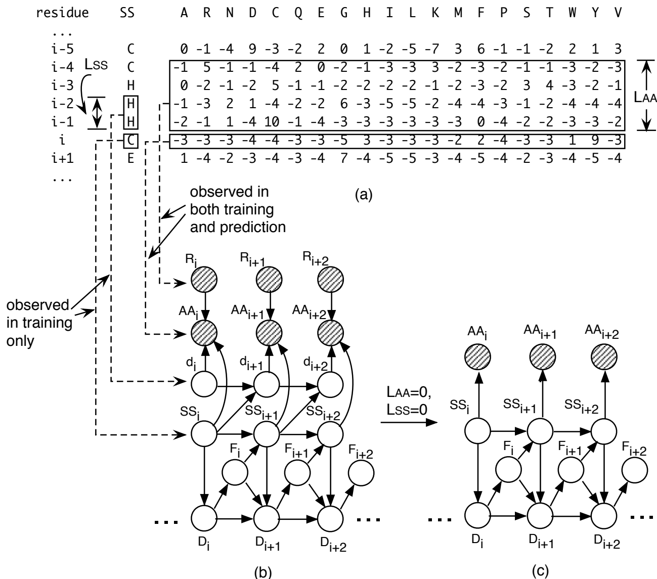
Figure 2 Illustration of the DBN model. (a) An example of PSSM, where rows represent residue sites and columns represent amino acids. The "SS" column contains the secondary structure of each site, classified as H (helix), E (sheet), and C (coil). (b) A graphical representation of the DBN. The shadow nodes represent observable random variables, while clear nodes represent hidden (in prediction) variables. The arcs with arrows represent dependency between nodes. The contents of the nodes R_i, AA_i, d_i , and SS_i are derived as illustrated by the connections of dashed lines, where the subscript indicates the residue site. More detailed description of R_i, AA_i, d_i, SS_i, D_i , and F_i can be found in the text. L_{AA} and L_{SS} are windows for profile and secondary structure, respectively (in this example, L_{AA} = 4 and L_{SS} = 2 ). (c) Is a reduced version of (b) with L_{AA} = 0 and L_{SS} = 0 .
