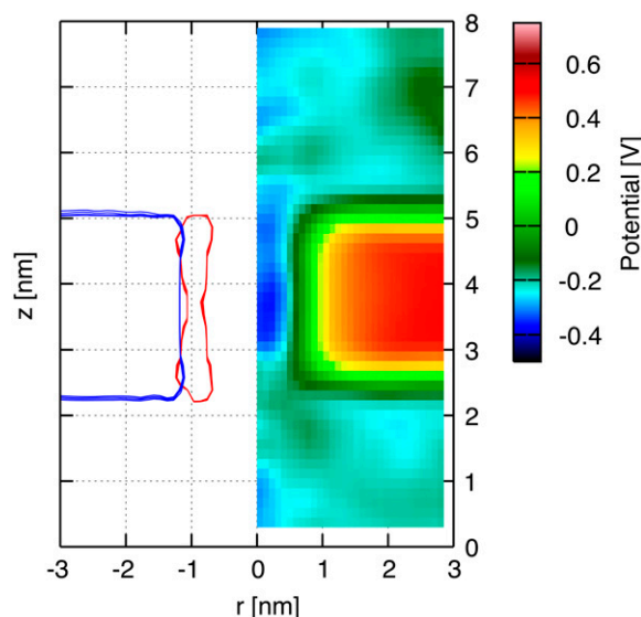
FIGURE 2 Radially averaged electrostatic potential map ( right ) and density profile ( left ) on the (r, z) plane for a CNT in a dodecane membrane and in the absence of an imposed transmembrane potential difference. The radially averaged density profile indicates the dodecane molecules ( blue ) and the CNT ( red ).
