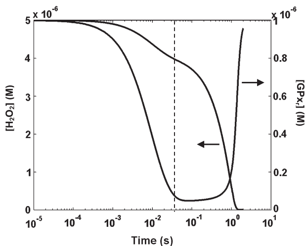
Figure 5. Example of the rate-limiting effect of the slower GPx r recycling step. Concentration profiles of H 2 O 2 and GPx r of the general model are shown for [H 2 O 2 ] 0 of 5 μM, [GSH] 0 of 0.1 mM and [GPx r ] 0 of 1 μM. The inflection point on the [H 2 O 2 ]-profile that occurs around 40 ms corresponds to the change in the rate of production of GPx r .
