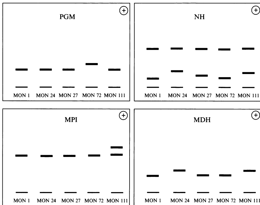
Fig. 5. Diagram showing the relative electrophoretic mobility of four isoenzyme markers for the main Leishmania infantum zymodemes found in Italy (PGM, phosphoglucumylatase; NH, nucleoside purine hydrolase; MPI, mannose phosphate isomerase; MDH, malate dehydrogenase). The zymodemes show identical mobility in the remaining nine enzymes examined. Montpellier (MON) 1, MON 27 and MON 72 are the main cause of visceral leishmaniasis, while MON 24 and MON 111 are common agents of cutaneous leishmaniasis in HIV-negative subjects [2]. Note that MON 72 differs from MON 1, the commonest L. infantum zymodeme, only in the mobility of PGM.
