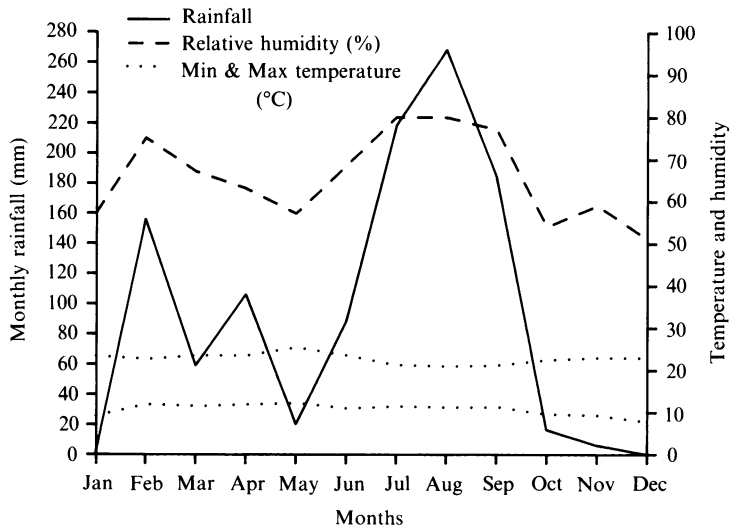
Fig. 2. Meteorological data of Addis Ababa, 1990.
