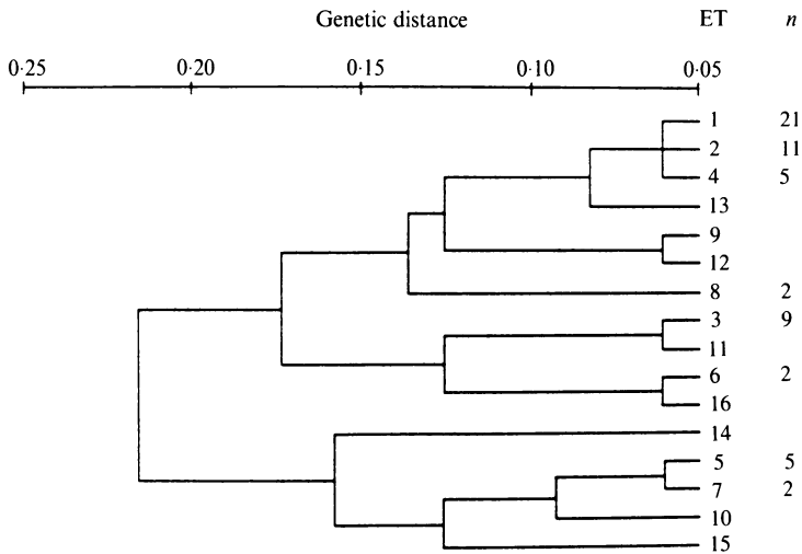
Fig. 1. Genetic relationships among the 16 ETs of Neisseria gonorrhoeae . The dendrogram was generated by the average-linkage method of clustering from a matrix of coefficients of pairwise genetic distance based on ten enzyme loci. The number of isolates ( n ) in each ET represented by multiple isolates is indicated.
