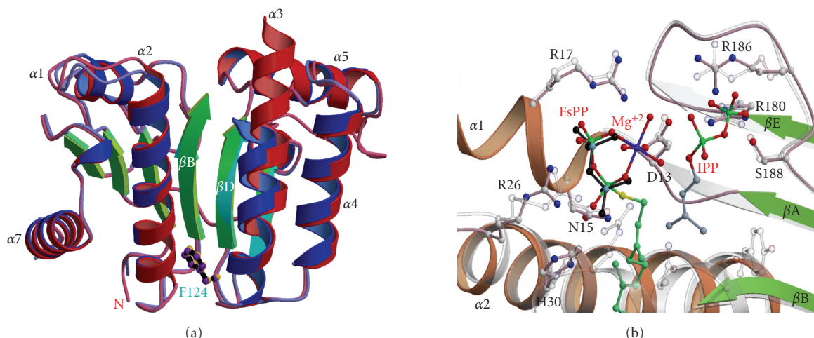
FIGURE 1: Crystal structures of H. pylori UPPS. (a) Two subunits of the apoenzyme are superimposed. The most obvious disposition occurs in \alpha 3 helix which adopts an open form and a closed form in subunit A and B, respectively. At the top of the tunnel-shaped crevice surrounded by 2\alpha -helices and 4\beta -strands is the substrate-binding site. Phe124 located at the bottom of the H. pylori UPPS tunnel adopts a similar position to that of Leu137 in E. coli UPPS, essential for determining product chain length. (b) Superimposition of active site structures of H. pylori UPPS with FsPP and E. coli UPPS with FsPP, Mg^{2+} , and IPP [9]. The active site residues in H. pylori UPPS are shown in pink and those in E. coli UPPS in white for carbon-carbon bonds in ball-and-stick model. The thiopyrophosphate (visible in crystal structure) is shown in black, the nitrogen atoms and Mg^{2+} ion are shown in blue, and oxygen atoms are shown in red. Asp13 in H. pylori UPPS occupies a similar position to that of Asp26 in E. coli UPPS to coordinate with an Mg^{2+} for binding with the pyrophosphate leaving group of FPP.
