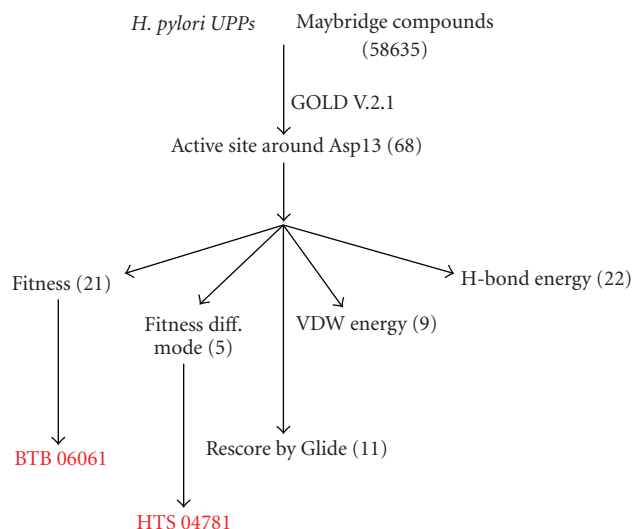
FIGURE 2: The flow chart for computer screening of H. pylori UPPS inhibitors. The active zone for screening was focused on Asp13, an important amino acid residue for coordinating with catalytic Mg^{2+} . In parentheses are the numbers of compounds. BTB06061 and HTS04781 are the final hits.
