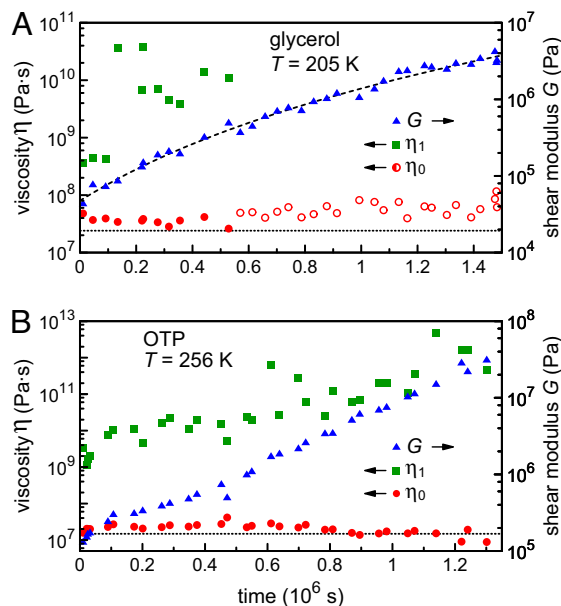
Fig. 3. Aging of glycerol and OTP. (A) Aging of the shear modulus G (right y -axis) and of the viscosity parameters \eta_0 and \eta_1 (left y -axis) of glycerol at 205 K as functions of time over a period of 2 weeks. Note that the system already presented a weak shear modulus at the beginning of the measurements. The values of the effective viscosity \eta_1 (squares) depend on the applied stress (see Fig. 4). The measurements up to 5 \times 10^5 s were done at a shear stress of 107 Pa (filled circles representing \eta_0 ), and later measurements at 213 Pa and 427 Pa (open circles). The dotted line corresponds to the viscosity derived from the liquid response at large stress, which is close to the literature value. The dashed curve, drawn through the shear modulus data points (triangles) as a guide to the eye, is a fit by a power law of time, G(\text{Pa}) = 10^{-18.5} \times [t(\text{s}) + 750,000]^{3.9} . (B) Aging of OTP over a period of 2 weeks at 256 K. The plot shows the evolution of the viscosities \eta_0 (circles, left y -axis) and \eta_1 (squares, left y -axis), as well as of the shear modulus G (triangles, right y -axis). The dotted line denotes the viscosity value derived from the liquid response during initial cooldown, which is in agreement with previous measurements.
