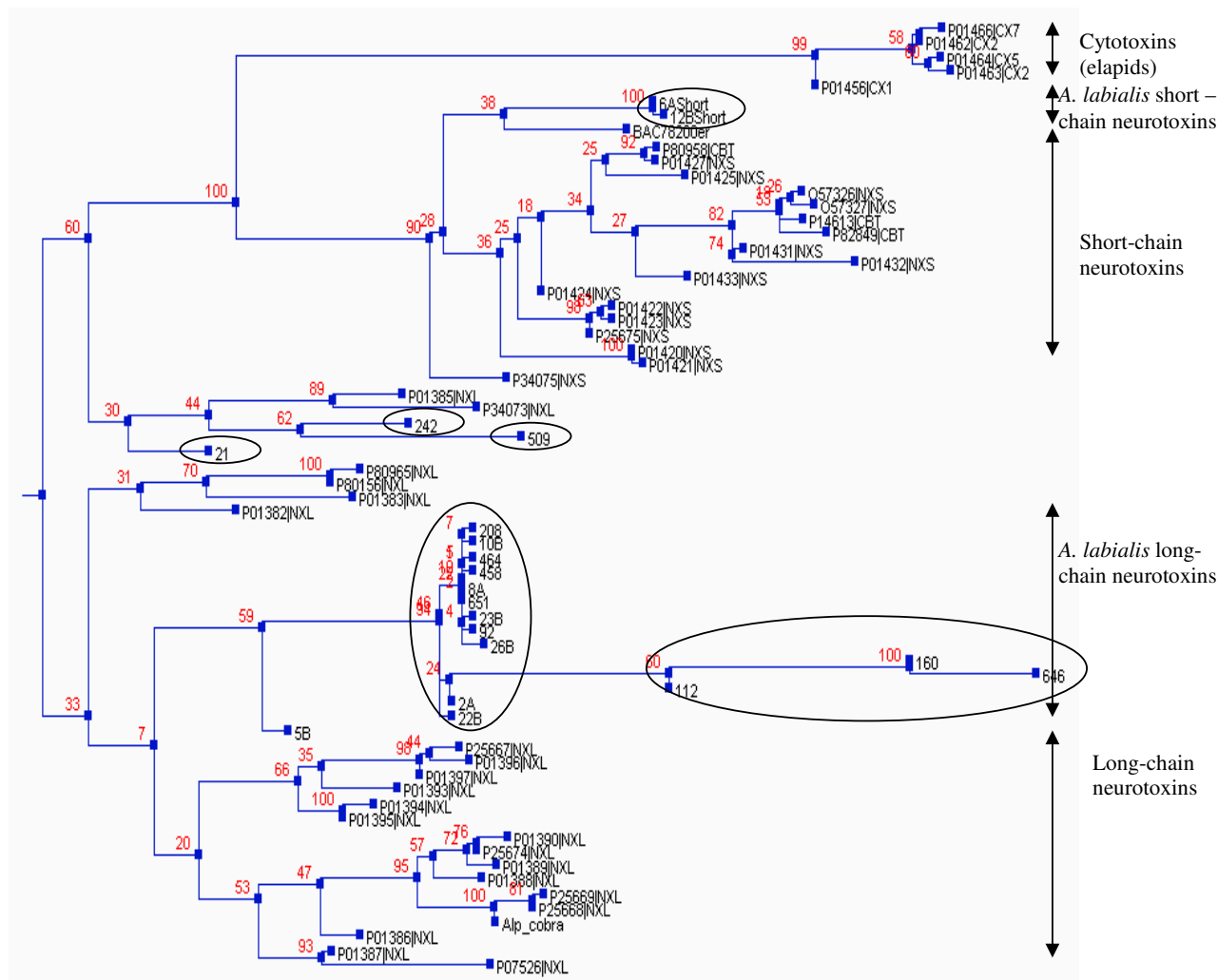
Figure 3 Phylogenetic tree of elapid three-finger toxins. Full length A. labialis long-chain and short-chain neurotoxins are encircled. Phylogram was generated by PHYML using maximum likelihood method.
