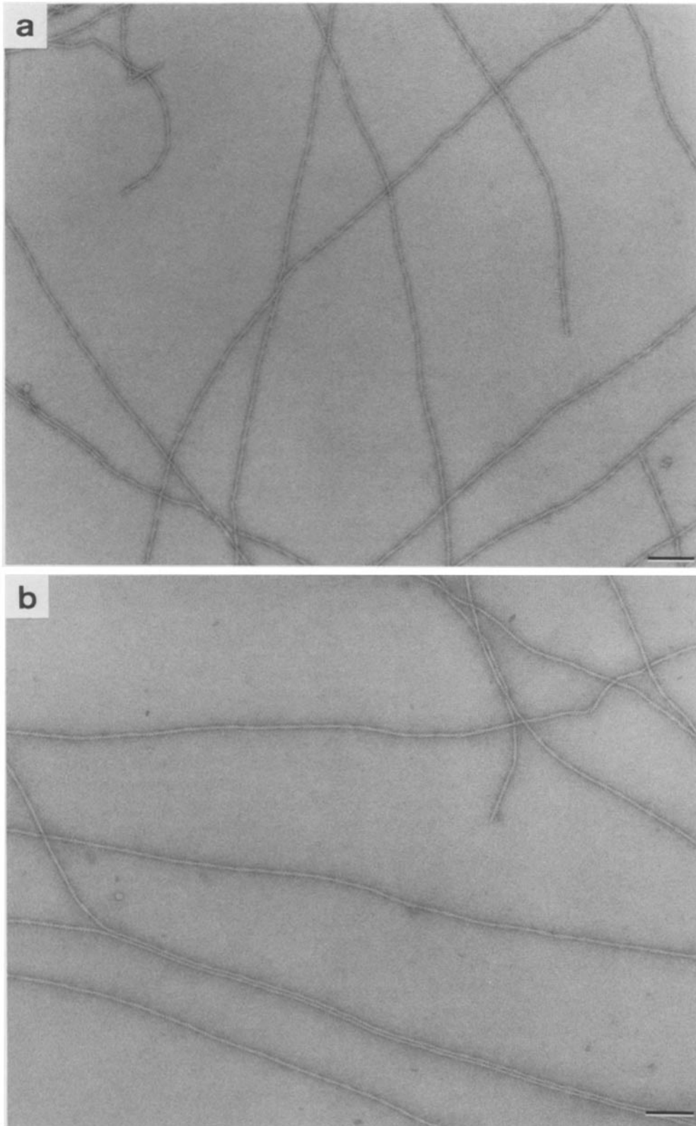
Figure 1. Electron micrographs of synthetic F-actin filaments negatively stained with 0.75% uranyl formate, pH 4.25. Rabbit skeletal muscle G-actin was polymerized ( a ) with 2 mM MgCl 2 /50 mM KCl and ( b ) with the same salts but in the presence of a 2:1 molar ratio of phalloidin to actin (see Materials and Methods). Bars: ( a and b ) 100 nm.
