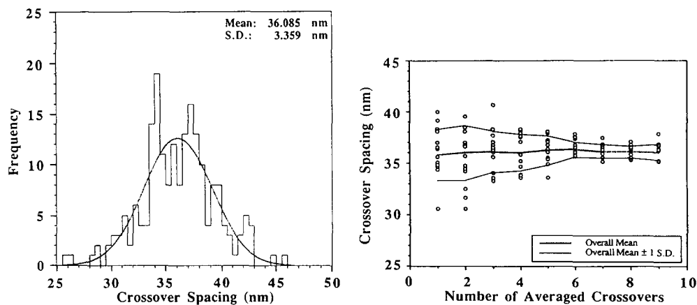
Figure 9. Comparison of the crossover spacing frequency distributions ( left panels ) and the running means along single filament stretches ( right panels ) for unstabilized F-actin filaments ( upper panels ) and phalloidin-stabilized F-actin filaments ( lower panels ). For the crossover spacing frequency distributions, 200 crossover values, each determined by the procedure outlined in Fig. 8, were included. Gaussian fits have been superimposed onto the histograms. For the running means, 13 9-crossover long filament stretches were analyzed for both unstabilized and phalloidin-stabilized filaments. Open circles represent the mean crossover spacing as a function of the number of crossovers averaged along the filament stretch (i.e., 1 to 9). The dotted line represents the overall mean (i.e., the average over all 13 values plotted) as a function of the number of crossovers averaged along the stretch, while the solid lines define an "envelope" function of overall mean \pm 1 SD.
