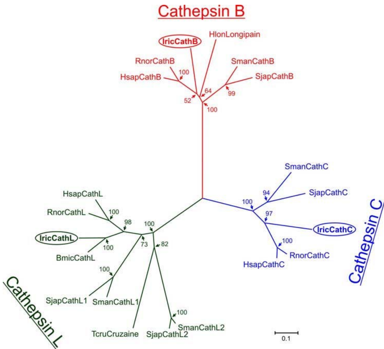
Figure 3 Phylogenetic relation of Ixodes ricinus gut-associated cysteine peptidases (clan CA, family CI) to selected representatives of the papain family. The tree was reconstructed by the Neighbor-joining method using amino acid sequences spanning across the homologous domains of mature enzymes. The horizontal bar represents a distance of 0.1 substitutions per site. Numbers at the branches display bootstrap support. Cathepsins B: Homo sapiens (AAH95408), Rattus norvegicus (P00787), Ixodes ricinus (ABO26563), Haemaphysalis longicornis (BAF43801), Schistosoma mansoni (P25792), Schistosoma japonicum (P43157); Cathepsins L: H. sapiens (M20496), R. norvegicus (AAH63175), I. ricinus (ABO26562), Boophilus microplus (AF227957), S. mansoni (CathL1 (Z32529), CathL2 (U07345)), S. japonicum (CathL1 (U38476), CathL2 (U38475)), Trypanosoma cruzii (P25779); Cathepsins C: H. sapiens (X87212), R. norvegicus (D90404), I. ricinus (ABV29335), S. mansoni (Z32531), S. japonicum (U77932).
