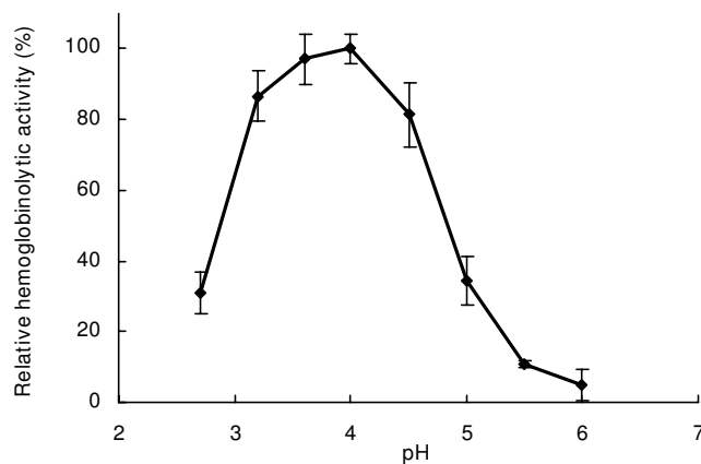
Figure 1 The pH profile of hemoglobinolytic activity in the I. ricinus gut tissue extracts. Gut tissue was dissected from partially engorged tick females (the 5-th day of feeding), washed from the gut contents and extracted. Fluorescently labeled AMC-hemoglobin was digested in vitro with gut extract at various pH values. The relative rate of degradation of the substrate was determined using the measurement of fluorescence in a continuous hemoglobinolytic assay. The error bars indicate standard deviations of the mean of triplicates.
