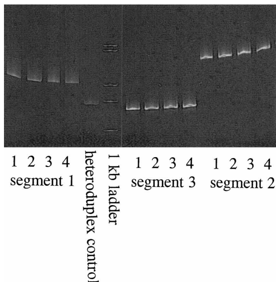
FIG. 5. PCR-heteroduplex analysis of three segments of the 16S rRNA genes of H. muris TR8556 (A), TR8563 (B), and TR8564 (C) amplified with three pairs of primers (segment 1, primers A-17mod and R385; segment 2, primers F312 and R768; segment 3, primers F1112 and EC9). The heteroduplexes of the three strains are as follows: lane 1, A and C; lane 2, A and B; lane 3, B and B; lane 4, B and C.
