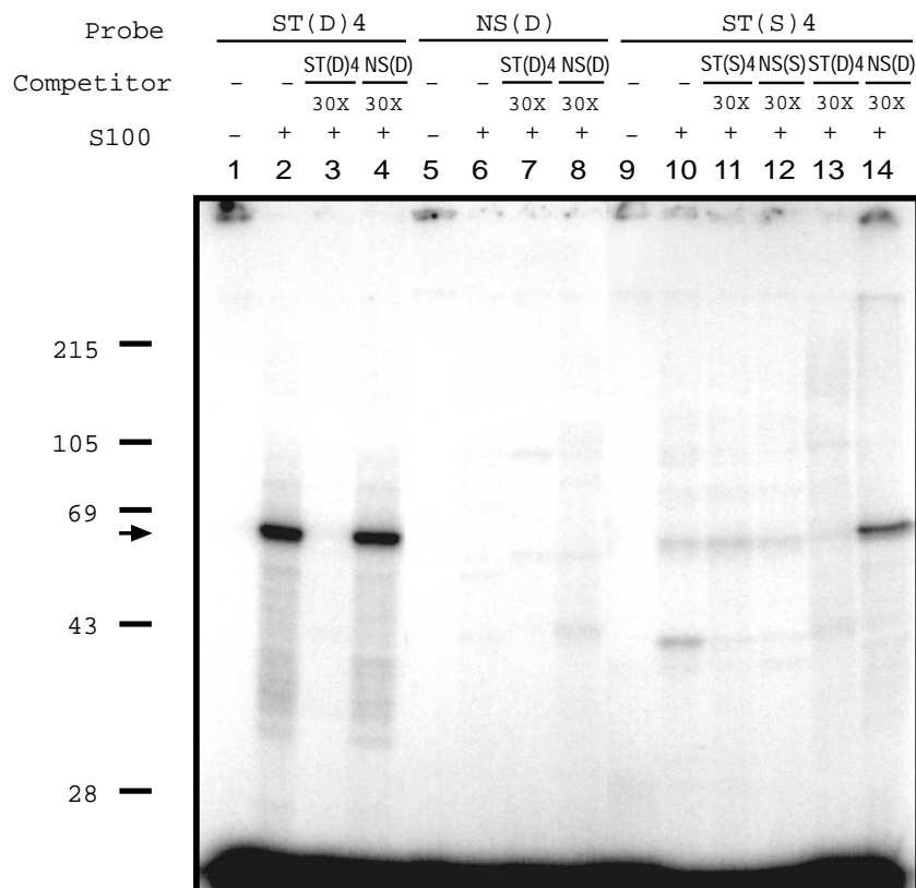
FIG. 8. UV cross-linking indicates a molecular mass for TEP of \sim 65 kDa. Radiolabeled ST(D)4 (lanes 1 to 4), NS(D) (lanes 5 to 8), or ST(S)4 (lanes 9 to 14) was incubated alone (lanes 1, 5, and 9) or allowed to bind TEP ( 6 \mu\text{g} of S100 extract from starved cells in lanes 2 to 4, 6 to 8, and 10 to 14) in the presence and absence of a 30-fold molar excess of various types of oligonucleotide competitors as indicated above the lanes. The reaction mixtures were irradiated with UV light and separated by SDS-PAGE. Protein size markers are indicated at the left in kilodaltons. The specific DNA-TEP complex revealed by SDS-PAGE is marked by an arrow. One microgram of unlabeled poly[d(I-C)] as a nonspecific competitor was present in all experiments.
