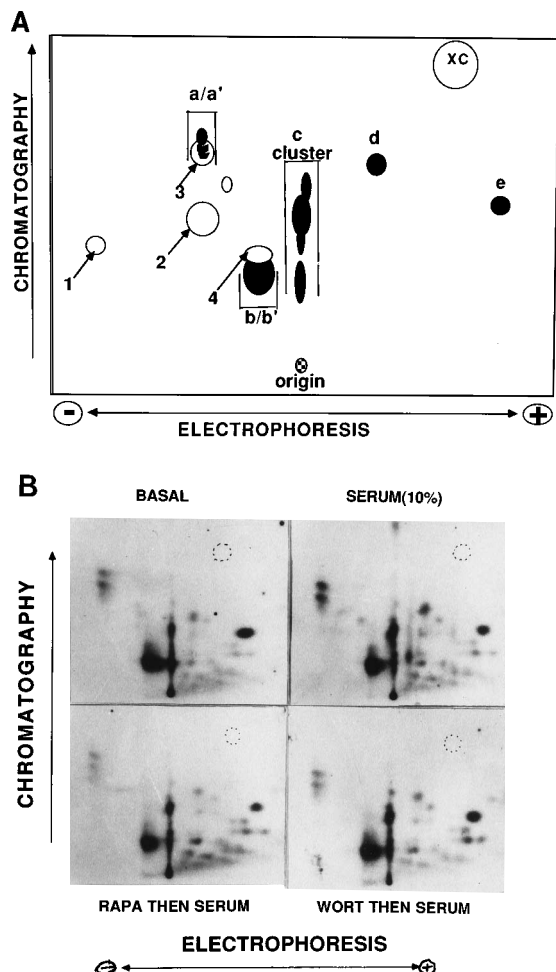
FIG. 4. 32 P-peptide maps of p70 S6 kinase. (A) Schematic representation of the 32 P-peptides visualized reproducibly in two-dimensional peptide maps of endogenous or recombinant p70 S6 kinase, 32 P labelled in NIH 3T3 cells, or during transient expression in 293 cells. The open symbols, which are numbered, are 32 P-peptides that are seen in full-length p70 but not in p70ΔCT104 (see Fig. 4B) and correspond to peptides that contain the phosphorylation sites in the SKAIPS domain (6, 12). The filled symbols, which are given letter designations, are seen in maps of both full-length p70 and p70ΔCT104. XC, xylene cyanol marker. (B) Autoradiographs of two-dimensional 32 P-peptide maps of digests prepared from the 32 P-labelled p70ΔCT104 polypeptides shown in the bottom panel of Fig. 1A. Aliquots containing equal (1,000) 32 P cpm were subjected to thin-layer electrophoresis (TLE)/thin-layer chromatography and the plates were all exposed for 3 days. RAPA, rapamycin; WORT, wortmannin.
