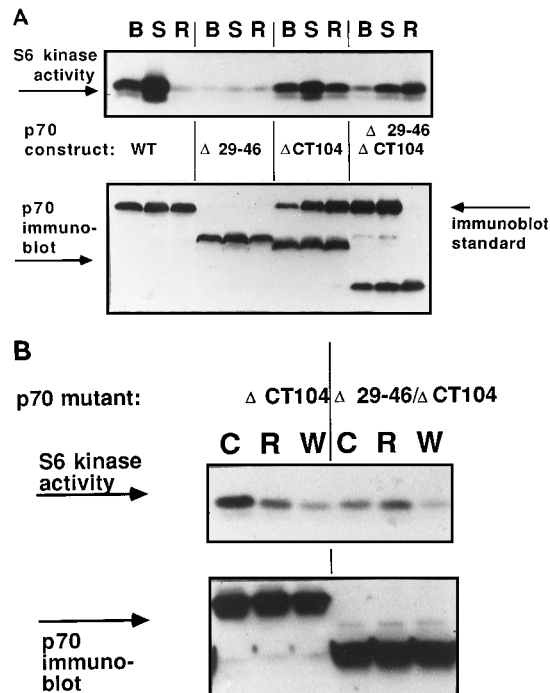
FIG. 3. Deletion of p70 residues 29 to 46 inhibits 40S kinase only if the p70 carboxy-terminal tail is present and greatly reduces rapamycin sensitivity. (A) The p70 variants indicated were expressed transiently in 293 cells as for Fig. 2. Serum-deprived cells were treated with basal medium (lanes B), 10% serum (lanes S), or rapamycin (10 nM) 15 min prior to serum addition (lanes R); extracts were prepared 20 min after serum addition; immunoprecipitation and the S6 kinase assay were performed as for Fig. 2. 40S kinase activities (picomoles per minute per unit of protein) for lanes B, S, and R, respectively, in this experiment were as follows: full-length (wild type [WT]), 1,780, 6,393, and 189; \Delta 29-46, 86, 145, and 168; \Delta CT104, 993, 2,887, and 932; \Delta 29-46/ \Delta CT104, 480, 1,333, and 1,253. These results were representative of three experiments. (B) Serum-replete 293 cells, transiently expressing p70 \Delta CT104 or p70 \Delta 29-46/ \Delta CT104, were treated with a maximally inhibitory concentration of rapamycin (50 nM, lanes R), a submaximally inhibitory concentration of wortmannin (100 nM; lanes W), or carrier (lanes C) for 15 min prior to harvest, immunoprecipitation, and assay of S6 kinase activity. The S6 kinase activities (picomoles per minute per unit of protein) for lanes C, R, and W, respectively, were as follows: p70 \Delta CT104, 444, 200, and 116; p70 \Delta 29-46/ \Delta CT104, 176, 220, and 91.
