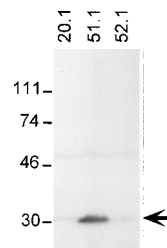
FIG. 7. The orfF gene product is overexpressed in strain LSB-51.1. Proteins from 5 × 10 7 cells of three strains of L. donovani (LSB-20.1, LSB-51.1, and LSB-51.2 [shown as 20.1, 51.1, and 52.1, respectively, over the lanes]), were separated by SDS-PAGE, transferred to nitrocellulose filters, and incubated with 1/200 dilution of rabbit antiserum against recombinant orfF protein. Bound antibody was visualized by incubation with 125 I-labeled protein A and autoradiography. The position of the predicted orfF gene product is indicated by the arrow. Molecular mass markers (Gibco-BRL) are shown to the left (in kilodaltons).
