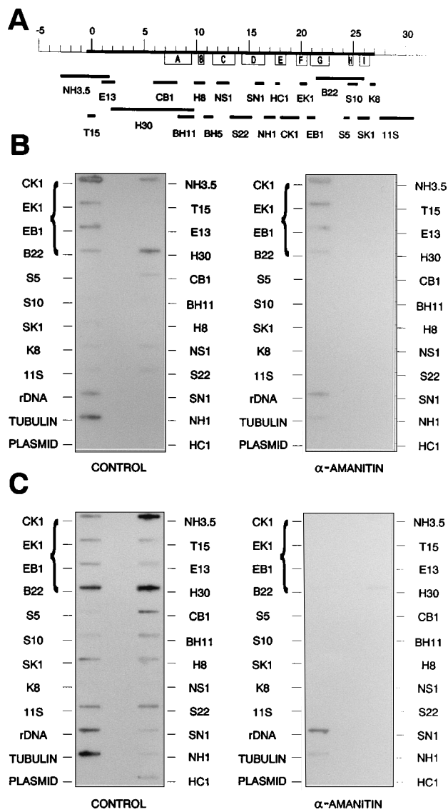
FIG. 6. The duplicated orfF and orfG in strain LSB-51.1 are transcribed by RNA Pol I. Samples (5 µg) of each plasmid clone representing various segments of the LD1 locus (A), T. brucei 18S rRNA genes (rDNA), T. brucei α- and β-tubulin genes (TUBULIN), and pBluescript II SK - (PLASMID) were blotted onto nylon membranes. Duplicate filters were hybridized with 32 P-labeled run-on transcripts from the nuclei of LSB-51.1 (B) or LSB-51.2 (C) labeled in the presence or absence (CONTROL) of 1 mg of α-amanitin per ml. Plasmid designations in the figure are shown minus the initial lowercase p.
