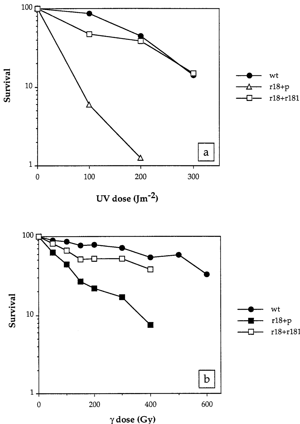
FIG. 5. Survival curves of rad18 and derivatives. (a) Cells (1,000) were plated and irradiated in a Stratalinker. Note that a Stratalinker reading of 100 \text{ J m}^{-2} appears to give a lower dose than indicated on the machine. (b) Cells in suspension were exposed to different doses of \gamma irradiation and then 1,000 cells were plated. wt, wild type; r18, rad18-X ; r18 + p, rad18-X transformed with pUR18N; r18 + r181, rad18-X transformed with rad18 gene in pUR18N (see text).
