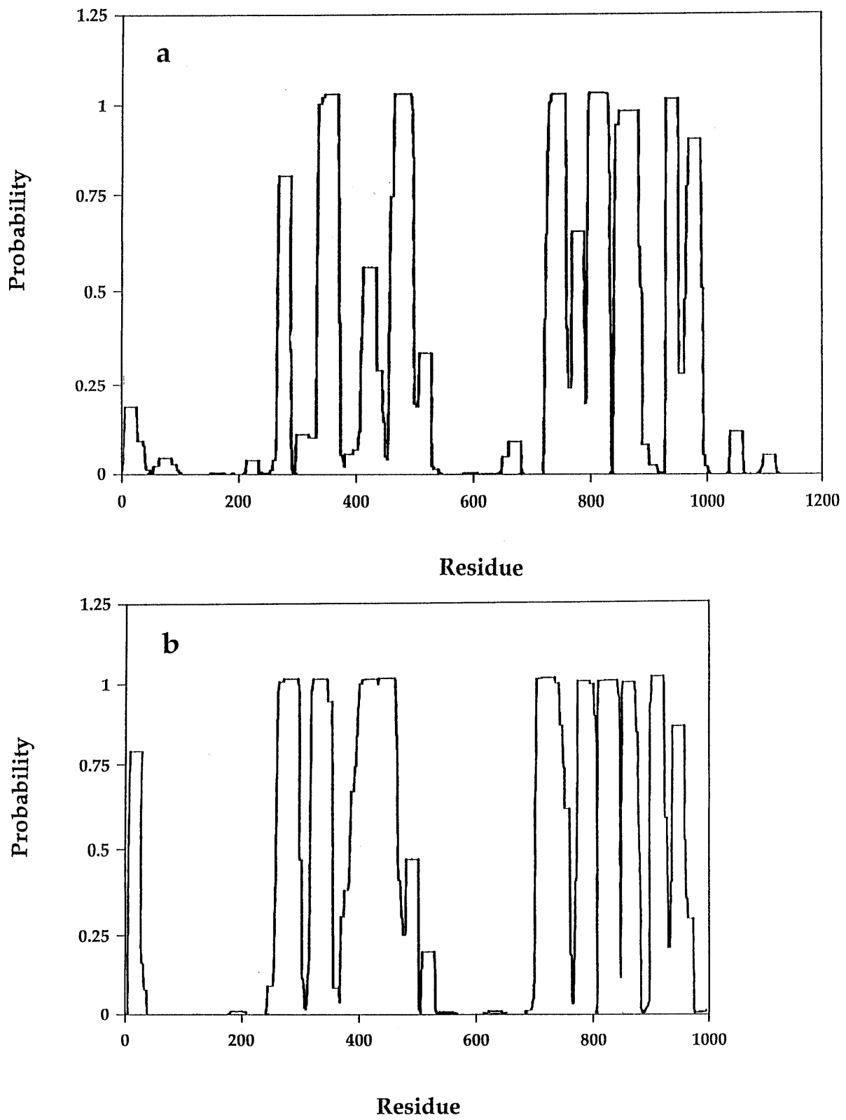
FIG. 7. Coiled coils in Rad18 (a) and Rhc18 (b). The protein sequences were analyzed by using the NewCoil program.
