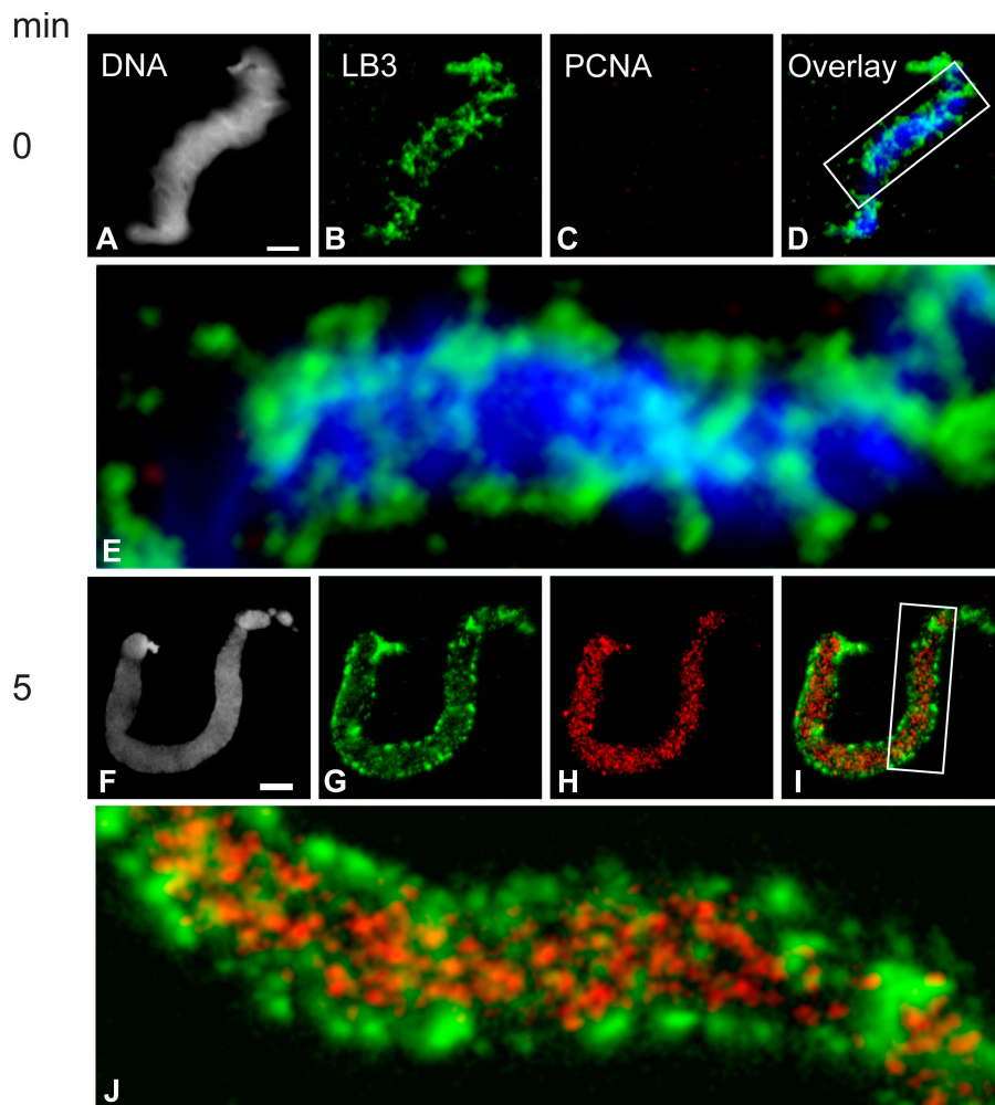
Figure 5. LB3 is present on demembrated sperm chromatin and is closely associated with PCNA during nuclear assembly. Demembrated sperm chromatin was exposed to hS, prepared for immunofluorescence with antibodies directed against LB3 and PCNA, and stained with Hoechst 33342 (A–E). Note that PCNA is absent, whereas LB3 is present and frequently appears to be helically wound around the chromatin (D and E). After the addition of X. laevis interphase extracts to sperm head chromatin for 5 min, LB3 is reorganized into patches and foci associated with chromatin (G, I, and J). In addition, PCNA is now present (H) and closely associated with LB3 (I and J). Enlargements of the regions in the boxes in the merged images (D, DNA and LB3; and I, LB3 and PCNA) are shown (E and J, 5.5× view). Bars, 5 μm. (K) The presence of LB3 and the absence of PCNA on demembrated sperm chromatin is also seen by immunoblotting. Demembrated sperm heads in the amount of 50,000 (lane 1), 100,000 (lane 2), or 200,000 (lane 3) were separated by SDS-PAGE, transferred to nitrocellulose, and probed for the presence of LB3 and PCNA. LB3 is seen in all lanes and is quantified relative to lane 3, but no PCNA could be detected.
