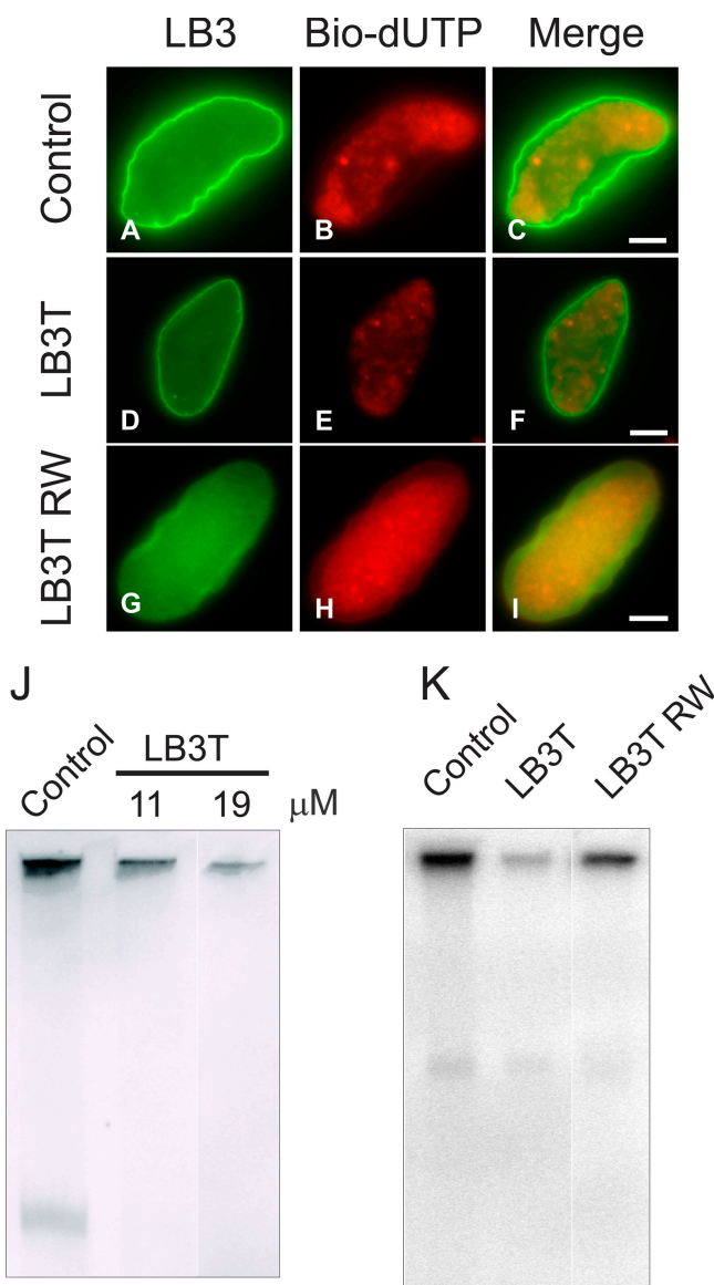
Figure 1. Addition of LB3T to assembled X. laevis nuclei inhibits DNA replication. Nuclei were assembled for 60 min followed by the addition of control buffer (A–C), \sim 19 \mu M LB3T (D–F), or \sim 19 \mu M LB3TRW (G–I) for 30 min followed by 5 \mu M bio-11-dUTP for 10 min. Nuclei were fixed, pelleted onto poly-L-lysine-coated coverslips, and prepared for immunofluorescence using Hoechst 33342, rhodamine avidin, and anti-LB3. Control nuclei continued to grow after addition of the buffer (A–C) and incorporated bio-11-dUTP (B). Using the same image capture settings, there was less incorporation of bio-11-dUTP after the addition of LB3T (E), and the nuclei appeared to be the same size as those in buffer controls at 60 min. In contrast, LB3T RW had a lesser effect on incorporation of bio-11-dUTP (H). (J) X. laevis nuclei were assembled for 60 min and different amounts of LB3T were added for 30 min followed by a 10-min incubation in 2 \mu C [ ^{32} P] \alpha -dCTP. The reactions were stopped by the addition of replication sample buffer for 10 min. The samples were run on 0.8% agarose gels and dried under vacuum, and radioactivity was measured. Under these conditions, there was a concentration-dependent inhibition of DNA replication attributable to LB3T. When \sim 11 \mu M LB3T was added, there was an \sim 50\% decrease, and with \sim 19 \mu M LB3T, replication decreased by \sim 92\% . (K) We also tested the effect of LB3T RW and determined that at a concentration of \sim 19 \mu M, DNA replication was reduced by \sim 50\% . Each experiment was repeated three times and the results were averaged.
