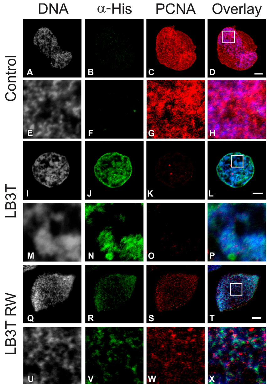
Figure 2. LB3T inhibits the association of PCNA with chromatin. X. laevis nuclei were assembled for 60 min before the addition either in the absence (A–H) or presence (I–P) of \sim 19 \mu\text{M} His-tagged LB3T for 30 min. Nuclei were prepared for immunofluorescence using antibodies directed against His 6 and PCNA and stained with Hoechst 33342. Control nuclei displayed only background His staining (B, D, F, and H) and a significant amount of PCNA mainly associated with chromatin (C, D, G, and H). In nuclei exposed to LB3T, the His-tagged protein was associated with chromatin (I, J, L–N, and P) and there was a substantial decrease in the amount of PCNA staining (K, L, O, and P). LB3T RW was also associated with chromatin but to a lesser extent than LB3T (Q, R, T–V, and X). Nuclei treated in this manner also had a reduced amount of PCNA associated with chromatin (S, T, W, and X). E–H, M–P, and U–X are 5x views of the boxes in D, L, and T. Bars, 5 \mu\text{m} .
