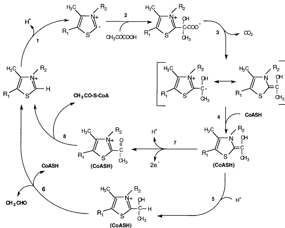
FIG. 5. Proposed catalytic mechanism of pyruvate decarboxylation under different conditions. See text for details.
