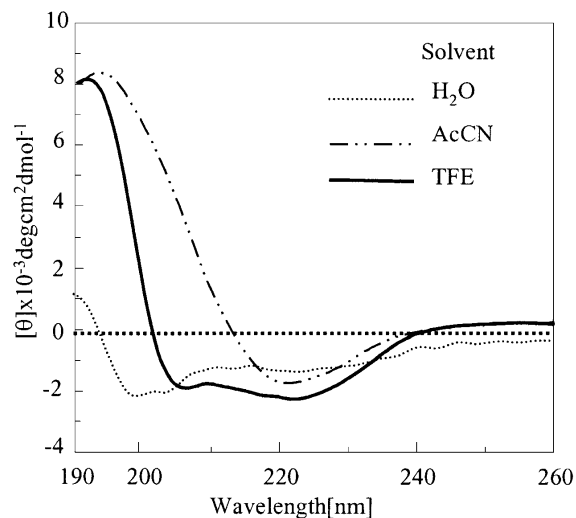
Figure 7. Solvent-dependent conformational transitions of Q 12 HQHQ 12 HQHQ 12 (disaggregated). In aqueous buffer the peptide displays an unordered structure (dotted line), presence of TFE results in an \alpha helical (solid line), whereas acetonitrile provides a \beta conformation (dot, dash line).
