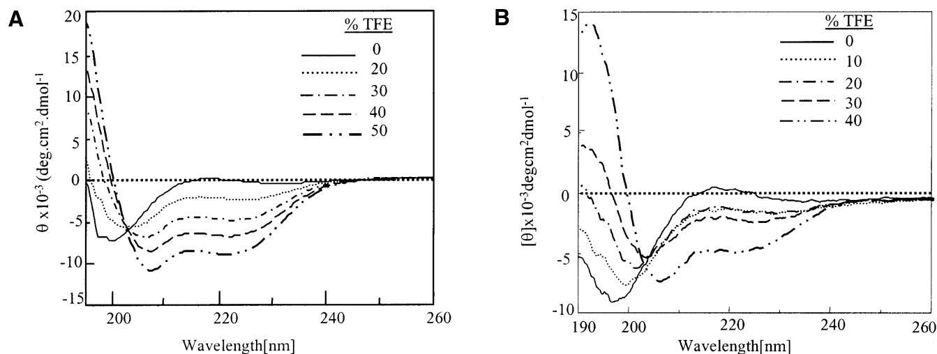
Figure 6. Effect of TFE on disaggregated (unordered) Q 12 HQHQ 12 HQHQ 12 and Q 8 PQPQ 8 . (A) Data indicate that Q 12 HQHQ 12 HQHQ 12 adopts sufficient helical character at 50% TFE (dot, dash line). (B) Q 8 PQPQ 8 adopts sufficient helical conformation at 40% TFE concentration (dash, dash line) with a sharp minimum at 208 nm.
