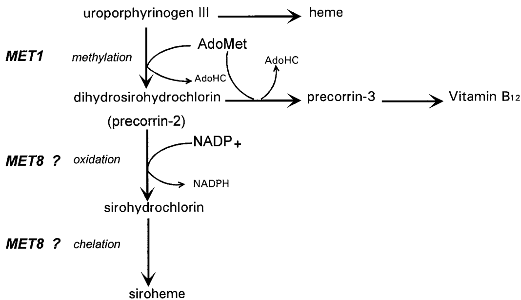
FIG. 6. Siroheme biosynthesis (88, 260).
