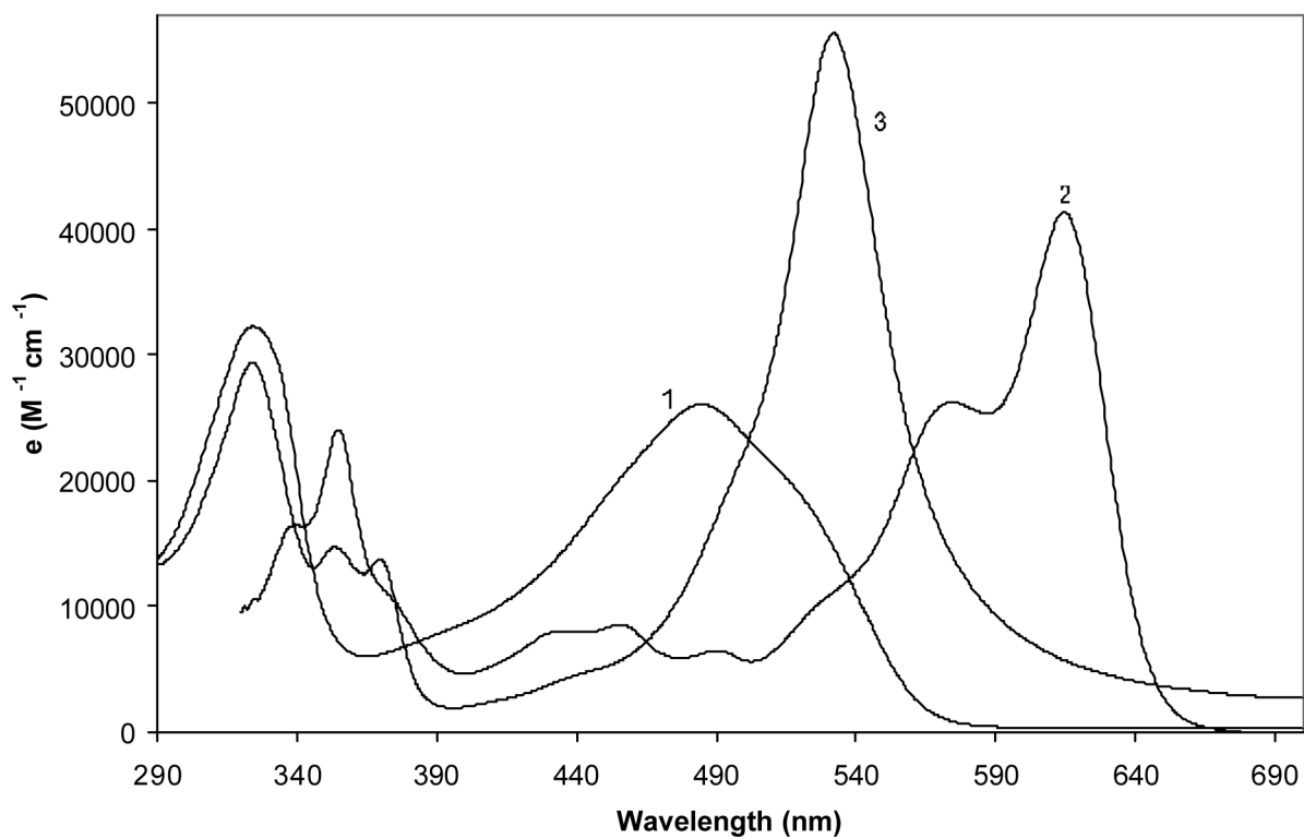
Figure 6. Influence of acid (curve 3: trifluoroacetic acid, neat) and base (curve 2: DBU, 1,8-diazabicyclo [5.4.0]undec-7-ene, neat) on the UV-visible spectra of 1 , compared with curve 1: CHCl 3 for \sim 1 \times 10^{-5} M solutions at 23°C.
