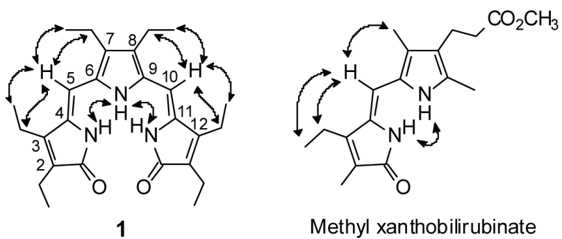
Figure 2. Nuclear Overhauser Effects (NOEs), indicated by curved arrows, seen in 1 in both CDCl 3 and (CD 3 ) 2 SO solvents. Similar NOEs are found in typical dipyrrirones, such as methyl xanthobilirubinate.
