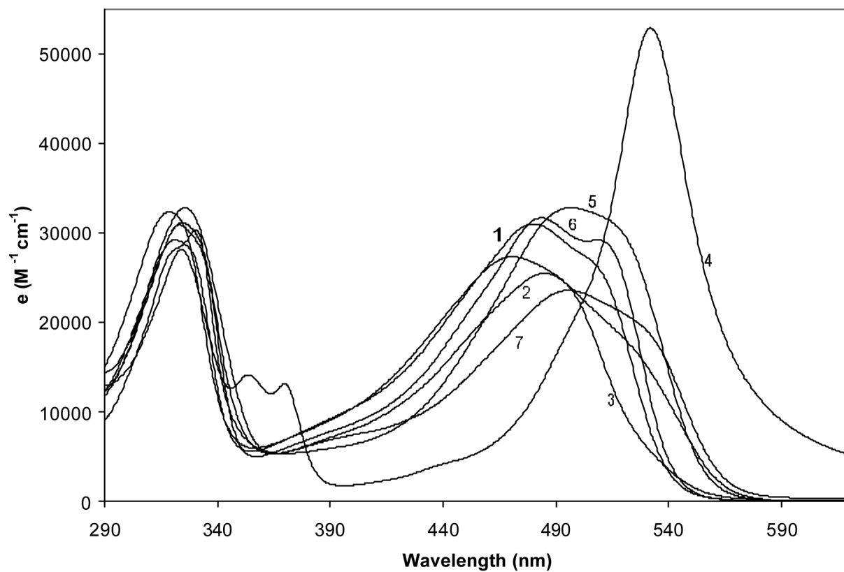
Figure 5. Solvent dependence of the UV-visible spectra of 1 at \sim 1 \times 10^{-5} M at 23°C. The curves are numbered corresponding to the solvents used: 1) methanol; 2) chloroform; 3) acetonitrile; 4) trifluoroacetic acid; 5) hexane; 6) dimethylsulfoxide; 7) benzene.
