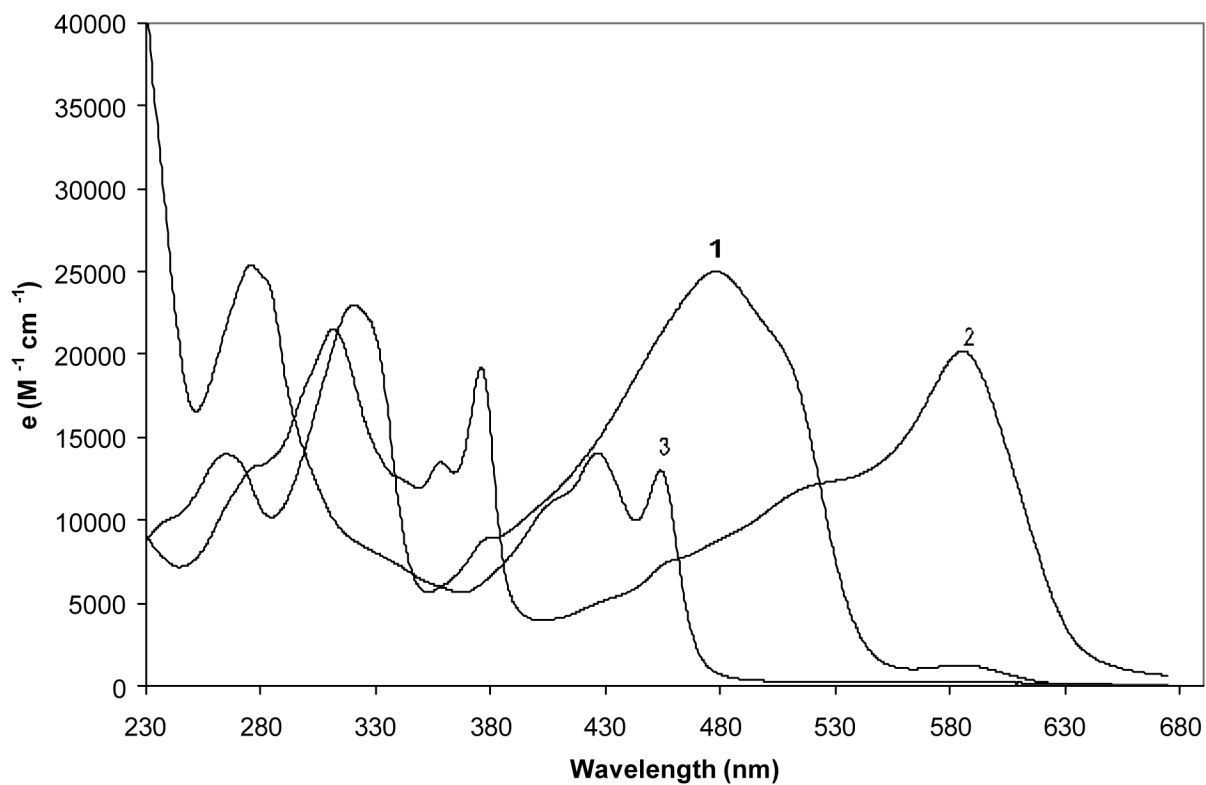
Figure 7. Influence of added zinc acetate (curve 2) followed by added conc. NH 4 OH (curve 3) on the UV-visible spectrum of 1 in CH 3 OH (curve 1) at \sim 1 \times 10^{-5} M concentration and 23°C.
