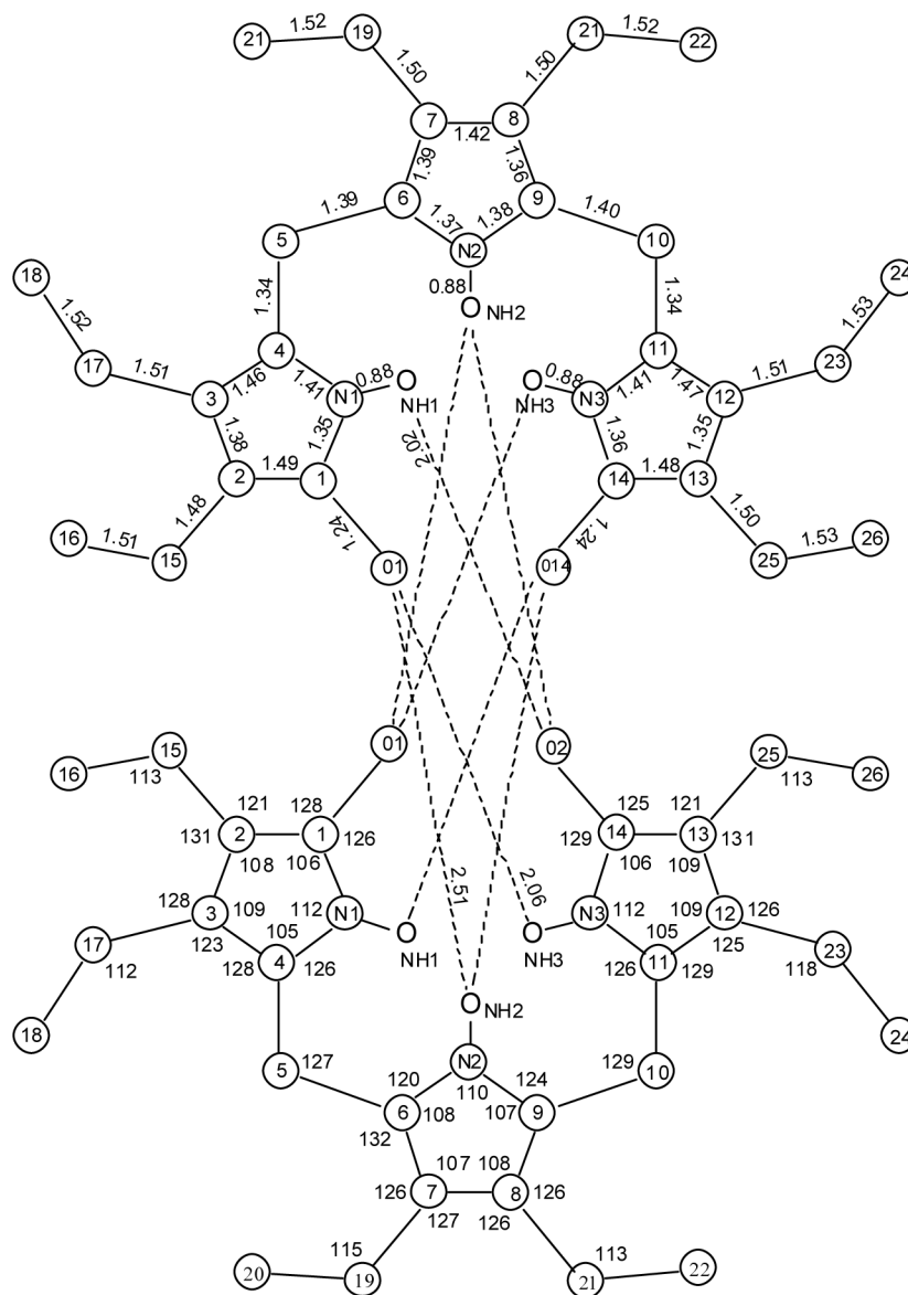
Figure 4. Bond distances (Å) and angles (°) found in the X-ray crystallographic structure of tripyrindione 1 hydrogen-bonded dimer, with numbering system used. Hydrogen bonding distances are indicated by dashed lines, and the following related main atom distances were found: O1-pyrrole N2 (3.19 Å), O1-lactam N3 (2.81 Å), O2-lactam N1 (2.84 Å). In a typical dipyrinone dimer X-ray crystal structure, 7,9-dimethyl-2,3,8-triethyl-10 H -dipyrinone (ref. 20), exhibits lactam O to pyrrole N and lactam O to lactam N distances: 2.89 Å and 2.86 Å, corresponding to pyrrole NH...O=C lactam distances of 2.09 Å and a lactam NH...O=C lactam distance of 2.09 Å and a lactam NH...O=C lactam distance of 1.97 Å. The bond lengths and bond angles are nearly identical.
