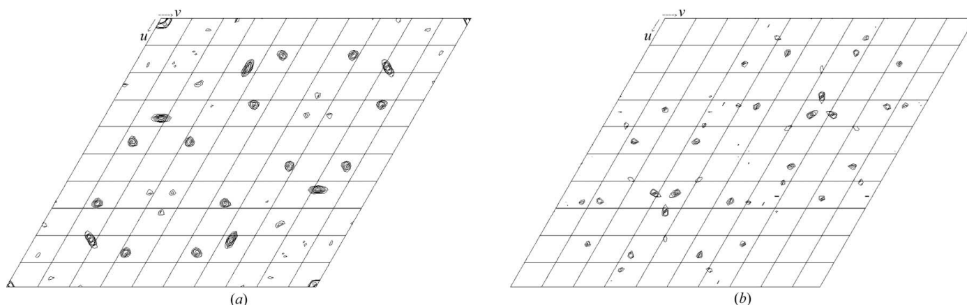
Figure 3 (a) Bijvoet and (b) dispersive difference Patterson maps ( w = 0.5 Harker section) calculated using the data from the SeMet derivative at 3.5 Å resolution. The contour lines are drawn from 2.5\sigma to 6.5\sigma , with an increment of 0.5\sigma .
