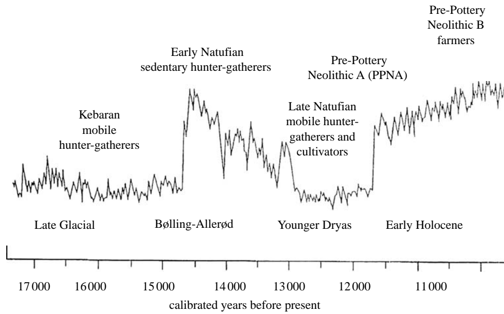
Figure 5. The environmental and cultural sequence of the southern Levant during the Late Pleistocene and Early Holocene. The line is based on oxygen isotope ratios used as a proxy for global temperature.
