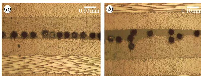
Figure 7. HGF spaced at 70\ \mu\text{m} showing (a) good embedment and (b) fibre clumping within host laminate.
