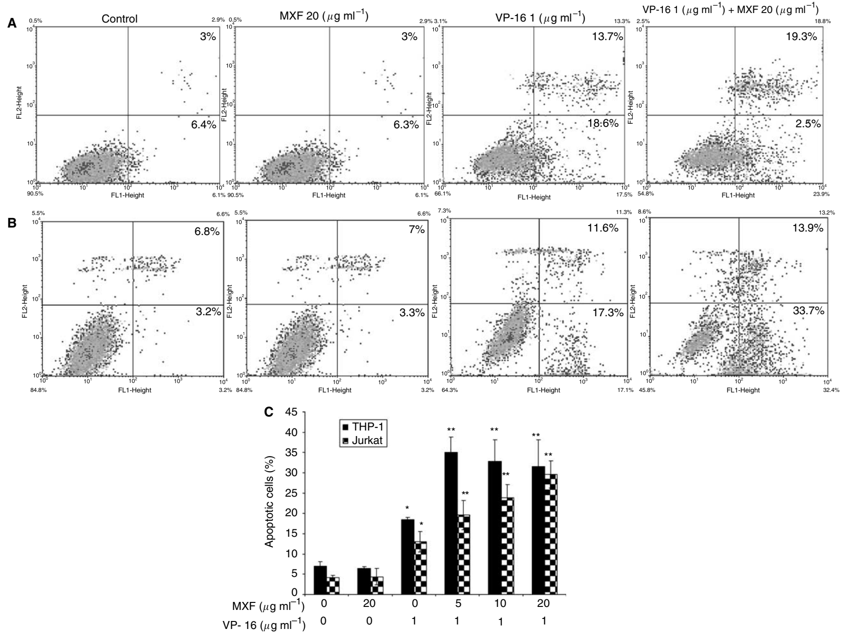
Figure 3 Moxifloxacin enhances apoptosis induced by VP-16. THP-1 (A and C) and Jurkat cells (B and C) were incubated for 24 h with VP-16 and MXF as indicated and flow cytometric analysis was performed by binding of annexin V and uptake of PI. A representative experiment is shown in (A and B). Results (mean \pm s.e.) of two independent experiments are shown in (C). The percentage of annexin V-positive, PI-negative cells is indicated in the lower right quadrangle and of annexin V-positive, PI-positive cells in the upper right quadrangle. The X-axis shows log annexin V fluorescence intensity and the Y-axis shows PI fluorescence intensity. * P < 0.04 for cells treated with VP-16 + MXF vs VP-16 alone.
