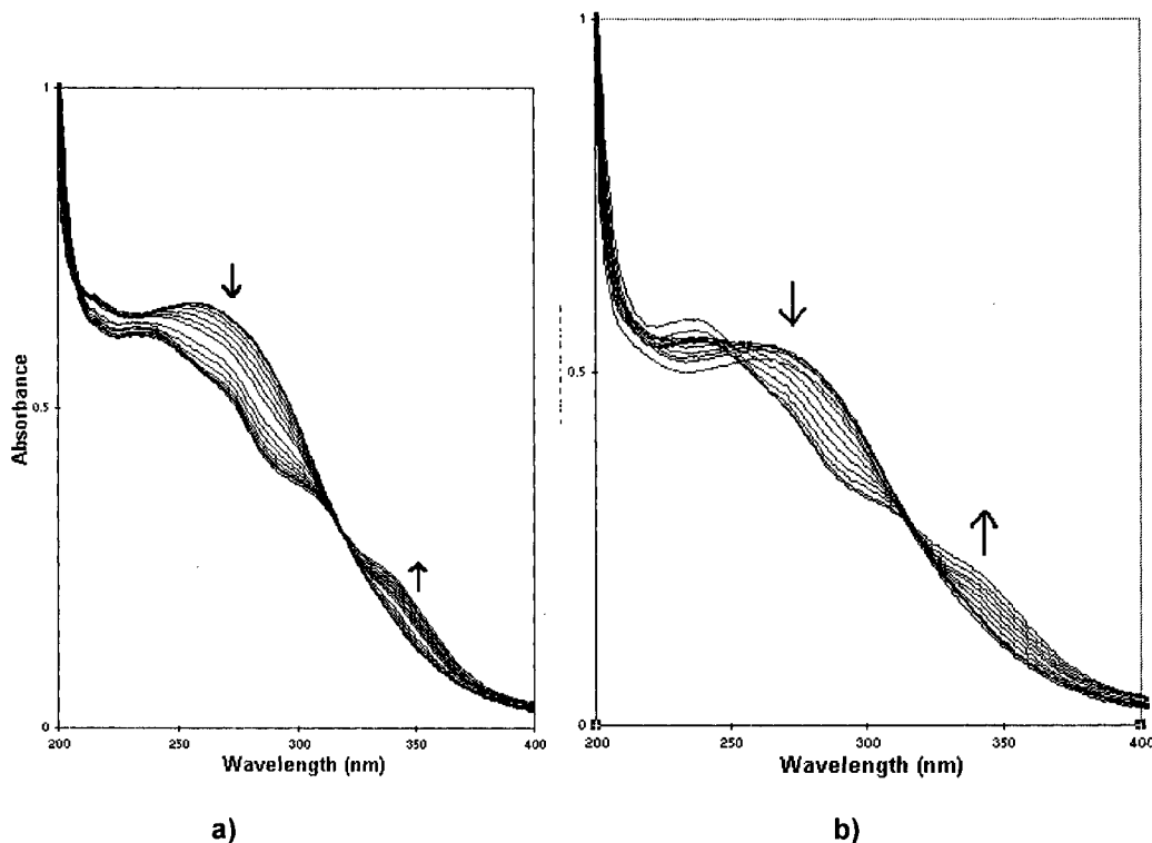
Figure 3 Ultraviolet absorption spectral changes for a) Fe-EDTA-bisamide and b) Fe-ADR-925 upon base titration. Iron complexes were 100 \mu M. The pH ranges were 4.0-6.9 for Fe-EDTA-bisamide and 4.2-8.2 for Fe-ADR-925. At higher pHs, the iron complexes become unstable toward iron hydroxide and oxide formation and precipitation.
