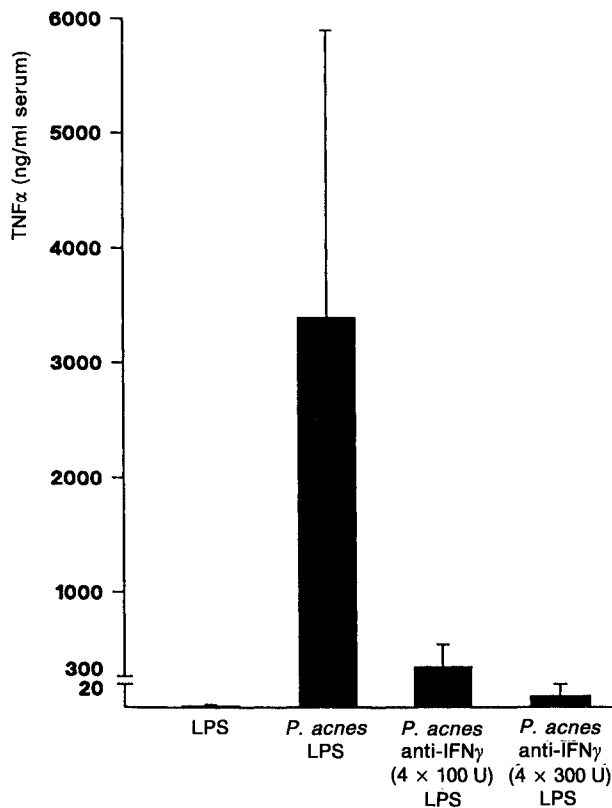
FIG. 3. Effect of anti-IFN \gamma on P. acnes induced sensitization to LPS. TNF \alpha production.
