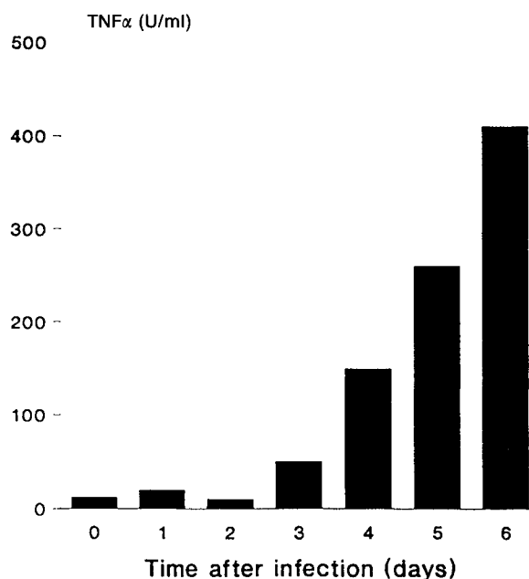
FIG. 1. Enhanced production of TNF \alpha by LPS in C3H/HeN mice infected with S. Typhimurium . Mice were infected with 50 CFU S. typhimurium and challenged with 10 \mu g LPS. Plasma was collected 60 min after LPS administration.
