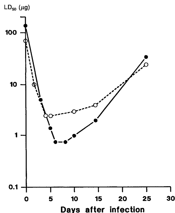
FIG. 2. Sensitization of mice to the lethal activity of LPS and HrTNF \alpha by sub-lethal infection with S. typhimurium . Mice (C3H/Tif) were infected with 2 \times 10^4 CFU of S. typhimurium and on different days thereafter groups were challenged with different amounts of LPS and the LD 50 values were calculated. ● LPS, ○ HrTNF \alpha .
