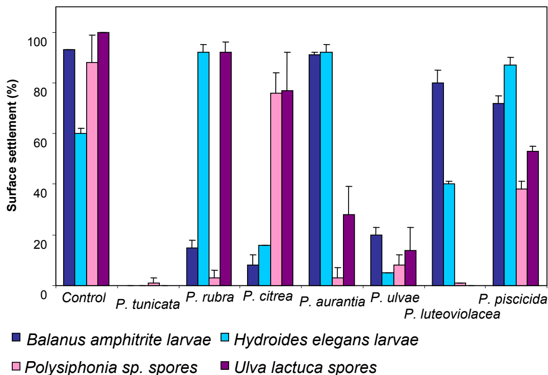
Figure 2. The inhibition of invertebrate larvae and algal spore settlement by different Pseudoalteromonas species. Data adapted from Holmström et al. [42].
