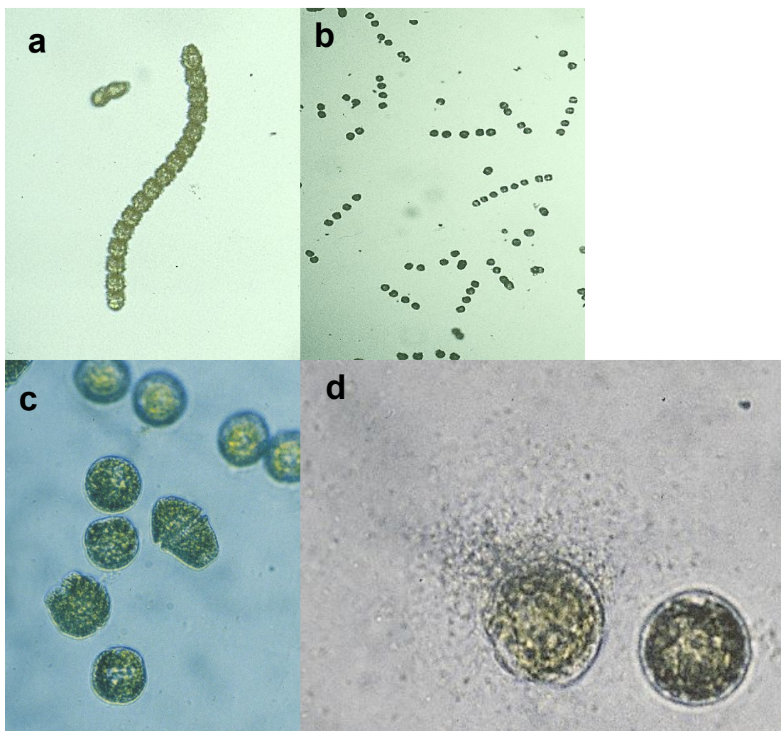
Figure 3. Anti-algal activity of Pseudoalteromonas species strain Y on the dinoflagellate Gymnodinium catenatum . a) Typical chain form of G. catenatum (time 0-10 minutes). b) Cell chains disassemble into individual cells (T=20 minutes); c) Cells become rounded (T=45 minutes); d) Cell lysis and leakage with strain Y swarming to a lysis cell (T=3 hours). Data and figures adapted from [92, 93].
