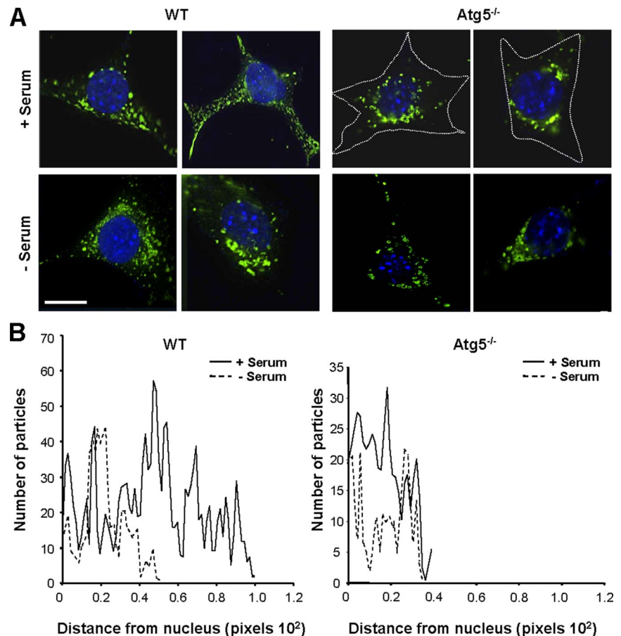
Figure 3. Relocation of CMA-active lysosomes toward the perinuclear region in Atg5 -/- cells. MEFs from WT and Atg5 -/- mice were maintained in the presence or absence of serum. After 12 h, cells were fixed and subjected to immunofluorescence for LAMP-2A. Mounting media contains DAPI to highlight the cell nuclei. (A) Representative cells for each condition. Discontinuous line marks the cellular perimeter in Atg5 -/- cells. Bar, 5 \mu m. (B) Quantification of the distribution of lysosomes (LAMP-2A-positive puncta) with respect to the nucleus in wild-type (left) and Atg5 -/- (right) MEFs under basal conditions and after serum removal. Values are mean of the quantification of 10 cells per condition in two independent experiments with two different WT and Atg5 -/- clones each. Mean cell size of Atg5 -/- cells was 1.3 + 0.2 times bigger than wild-type cells.
