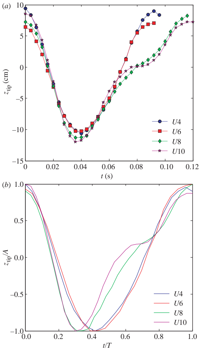
Figure 2. (a) Single typical wingbeats at flight speeds, U = 4, 6, 8 and 10 \text{ m s}^{-1} . (b) Wing traces of (a) normalized with amplitude, A , and stroke period, T , to illustrate the change in shape with U .
